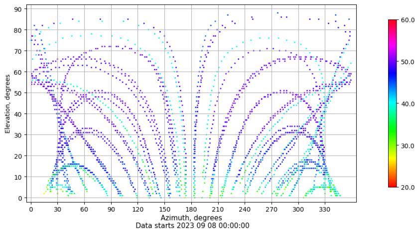
Azimuth-elevation plot for station ZFRA. Signal to Noise S1C Data file ZFRA00ESP_R_2023251.xtr
