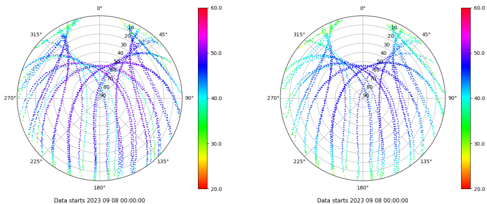
Skyplot for station ZFRA. Signal to Noise S1C Data file ZFRA00ESP_R_2023251.xtr Skyplot for station ZFRA. Signal to Noise S2P Data file ZFRA00ESP_R_2023251.xtr
