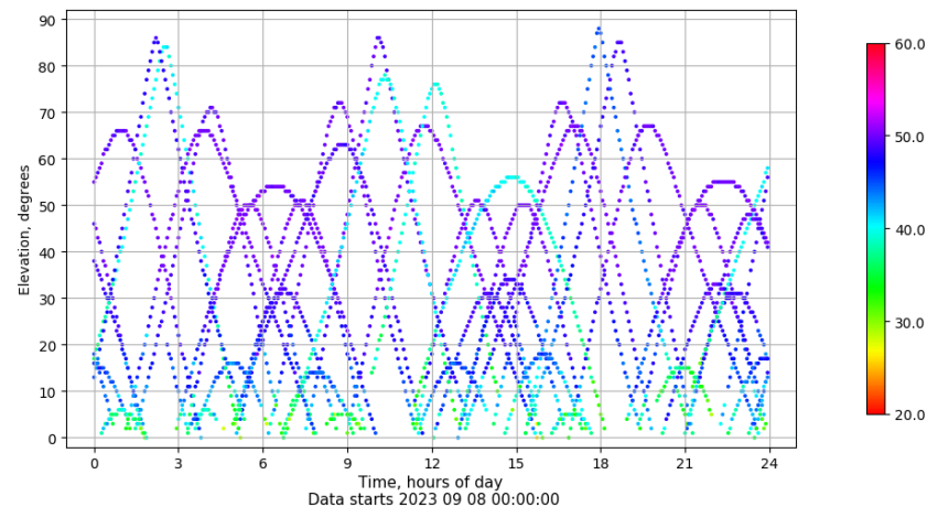
Time-elevation plot for station ZFRA. Signal to Noise S1C Data file ZFRA00ESP_R_2023251.xtr
