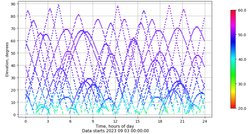
Time-elevation plot for station ZFRA. Signal to Noise S1C Data file ZFRA00ESP_R_2023246.xtr
