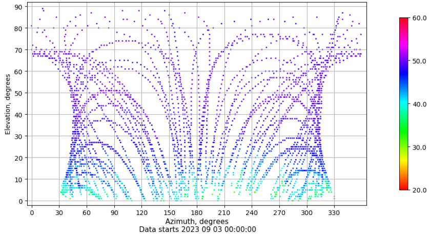
Azimuth-elevation plot for station ZFRA. Signal to Noise S1C Data file ZFRA00ESP_R_2023246.xtr
