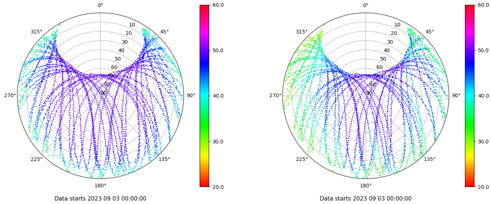
Skyplot for station ZFRA. Signal to Noise S1C Data file ZFRA00ESP_R_2023246.xtr Skyplot for station ZFRA. Signal to Noise S2W Data file ZFRA00ESP_R_2023246.xtr
