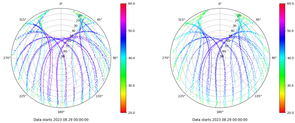
Skyplot for station ZFRA. Signal to Noise S1C Data file ZFRA00ESP_R_2023241.xtr Skyplot for station ZFRA. Signal to Noise S2P Data file ZFRA00ESP_R_2023241.xtr
