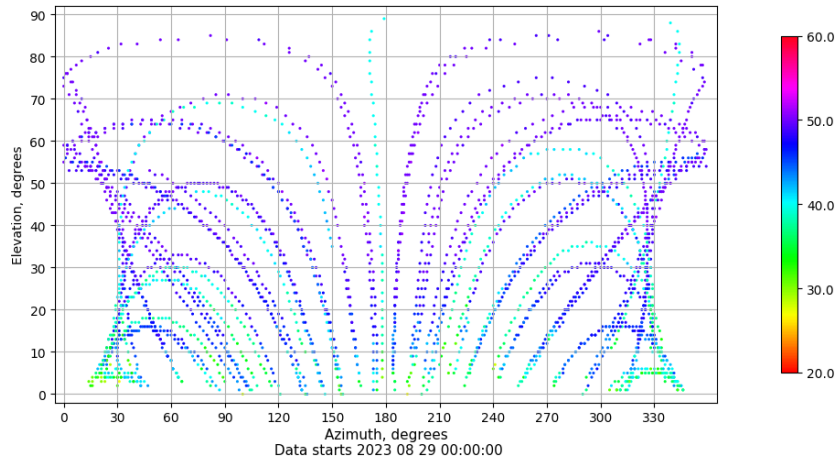
Azimuth-elevation plot for station ZFRA. Signal to Noise S1C Data file ZFRA00ESP_R_2023241.xtr
