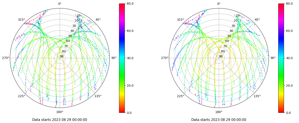
Skyplot for station ZFRA. Parameter M1C Data file ZFRA00ESP_R_2023241.xtr Skyplot for station ZFRA. Parameter M2P Data file ZFRA00ESP_R_2023241.xtr
