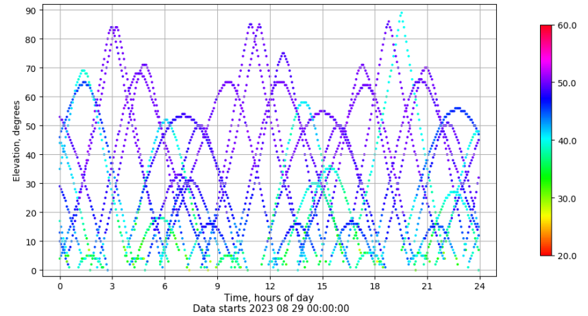
Time-elevation plot for station ZFRA. Signal to Noise S1C Data file ZFRA00ESP_R_2023241.xtr
