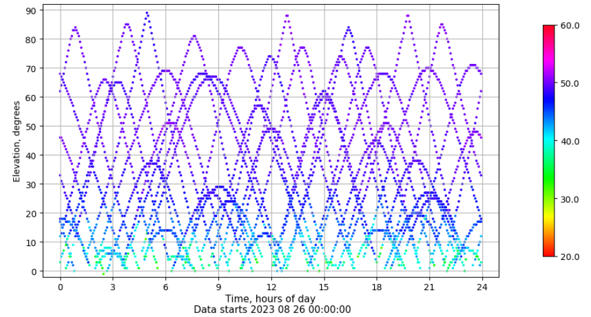
Time-elevation plot for station ZFRA. Signal to Noise S1C Data file ZFRA00ESP_R_2023238.xtr
