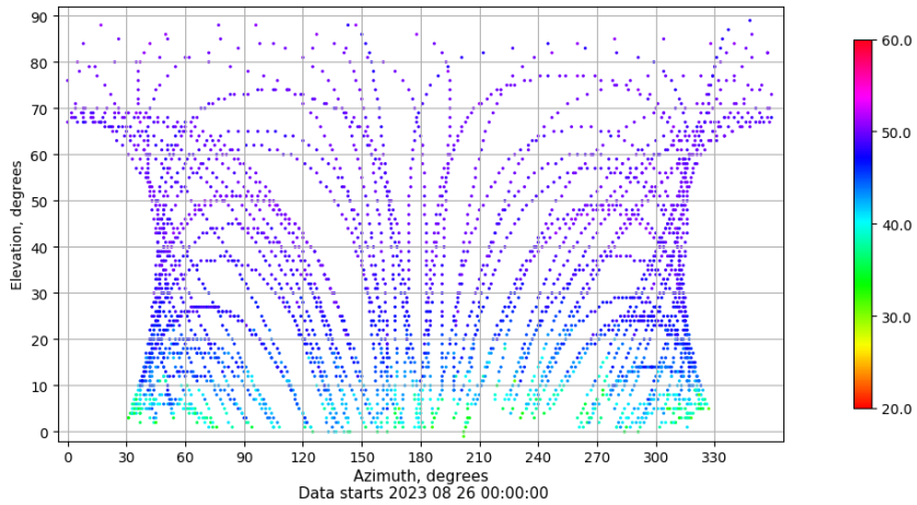
Azimuth-elevation plot for station ZFRA. Signal to Noise S1C Data file ZFRA00ESP_R_2023238.xtr
