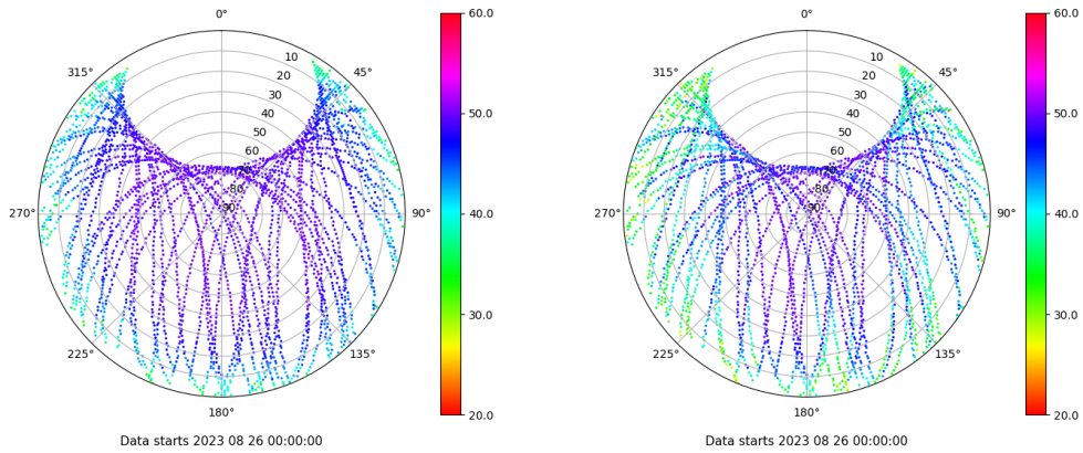
Skyplot for station ZFRA. Signal to Noise S1C Data file ZFRA00ESP_R_2023238.xtr Skyplot for station ZFRA. Signal to Noise S2W Data file ZFRA00ESP_R_2023238.xtr
