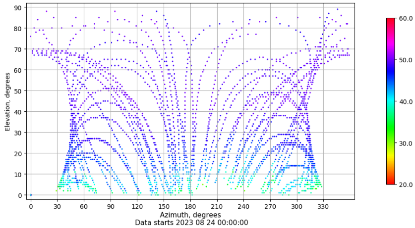
Azimuth-elevation plot for station ZFRA. Signal to Noise S1C Data file ZFRA00ESP_R_2023236.xtr
