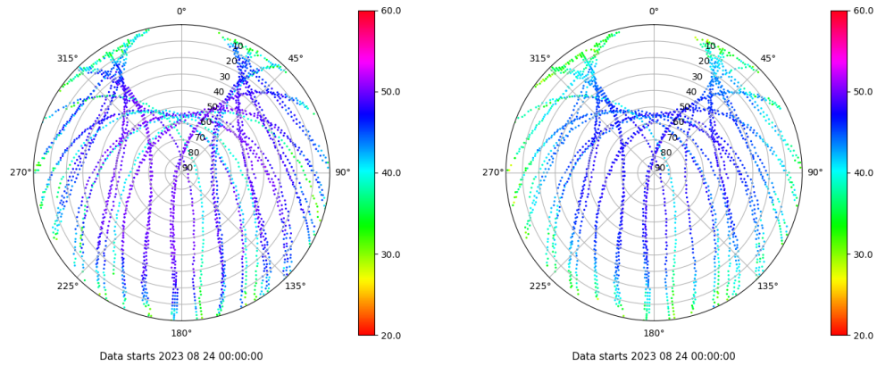
Skyplot for station ZFRA. Signal to Noise S1C Data file ZFRA00ESP_R_2023236.xtr Skyplot for station ZFRA. Signal to Noise S2P Data file ZFRA00ESP_R_2023236.xtr
