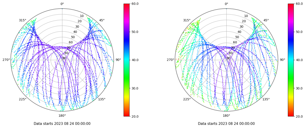
Skyplot for station ZFRA. Signal to Noise S1C Data file ZFRA00ESP_R_2023236.xtr Skyplot for station ZFRA. Signal to Noise S2W Data file ZFRA00ESP_R_2023236.xtr
