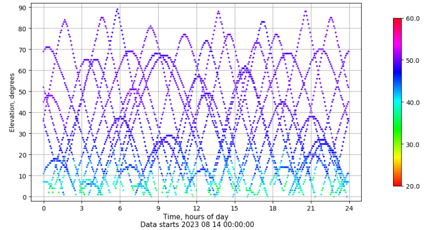
Time-elevation plot for station ZFRA. Signal to Noise S1C Data file ZFRA00ESP_R_2023226.xtr
