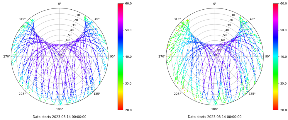
Skyplot for station ZFRA. Signal to Noise S1C Data file ZFRA00ESP_R_2023226.xtr Skyplot for station ZFRA. Signal to Noise S2W Data file ZFRA00ESP_R_2023226.xtr
