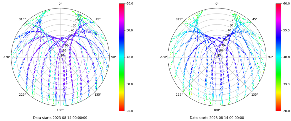
Skyplot for station ZFRA. Signal to Noise S1C Data file ZFRA00ESP_R_2023226.xtr Skyplot for station ZFRA. Signal to Noise S2P Data file ZFRA00ESP_R_2023226.xtr
