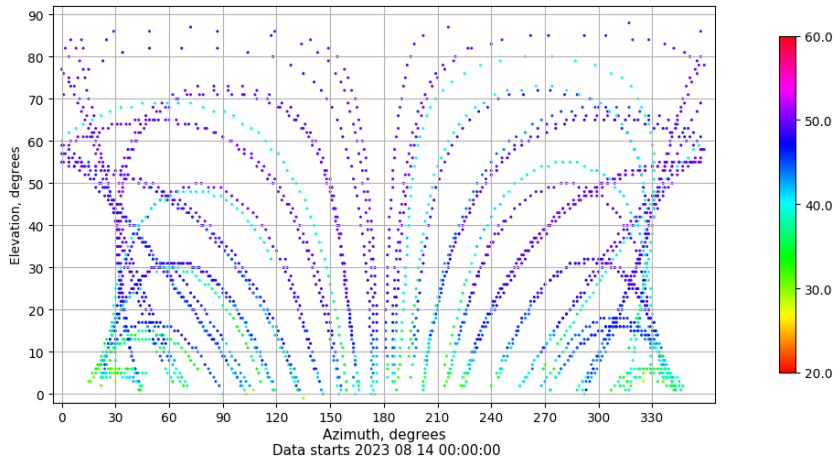
Azimuth-elevation plot for station ZFRA. Signal to Noise S1C Data file ZFRA00ESP_R_2023226.xtr
