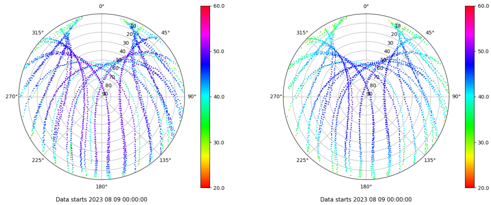
Skyplot for station ZFRA. Signal to Noise S1C Data file ZFRA00ESP_R_2023221.xtr Skyplot for station ZFRA. Signal to Noise S2P Data file ZFRA00ESP_R_2023221.xtr
