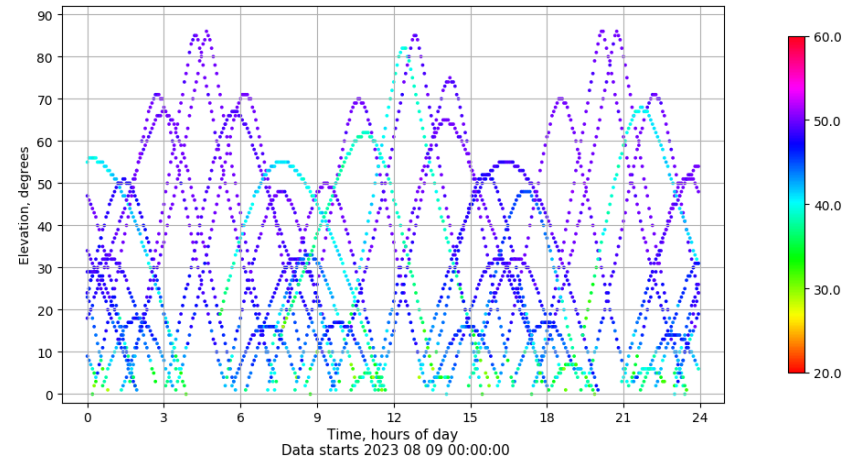
Time-elevation plot for station ZFRA. Signal to Noise S1C Data file ZFRA00ESP_R_2023221.xtr
