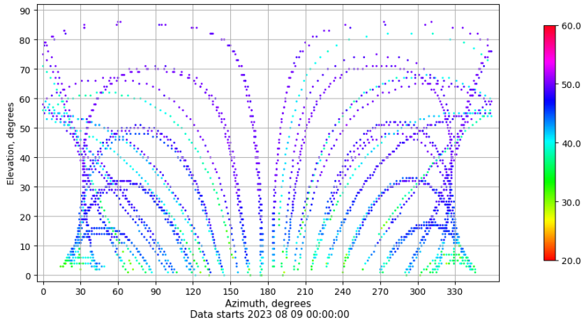
Azimuth-elevation plot for station ZFRA. Signal to Noise S1C Data file ZFRA00ESP_R_2023221.xtr
