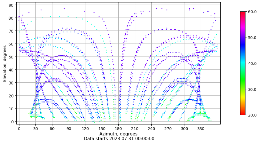
Azimuth-elevation plot for station ZFRA. Signal to Noise S1C Data file ZFRA00ESP_R_2023212.xtr
