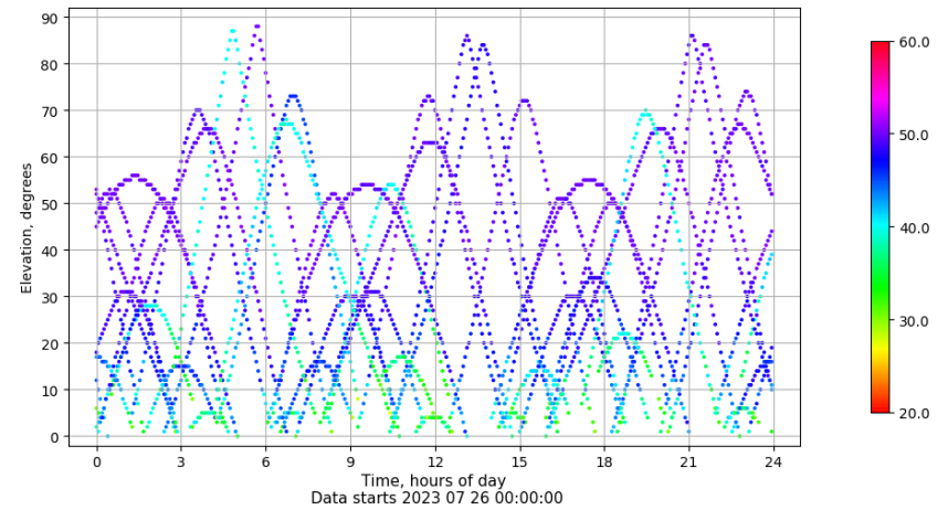
Time-elevation plot for station ZFRA. Signal to Noise S1C Data file ZFRA00ESP_R_2023207.xtr
