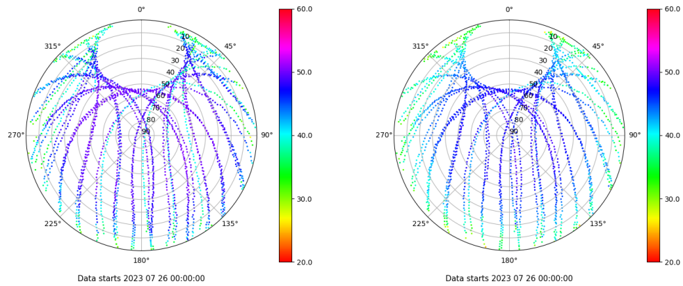
Skyplot for station ZFRA. Signal to Noise S1C Data file ZFRA00ESP_R_2023207.xtr Skyplot for station ZFRA. Signal to Noise S2P Data file ZFRA00ESP_R_2023207.xtr
