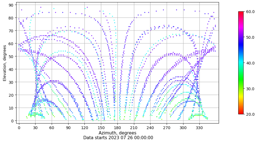
Azimuth-elevation plot for station ZFRA. Signal to Noise S1C Data file ZFRA00ESP_R_2023207.xtr
