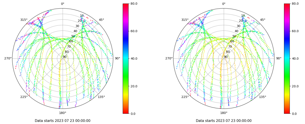
Skyplot for station ZFRA. Parameter M1C Data file ZFRA00ESP_R_2023204.xtr Skyplot for station ZFRA. Parameter M2P Data file ZFRA00ESP_R_2023204.xtr
