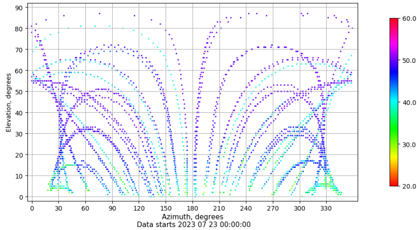
Azimuth-elevation plot for station ZFRA. Signal to Noise S1C Data file ZFRA00ESP_R_2023204.xtr
