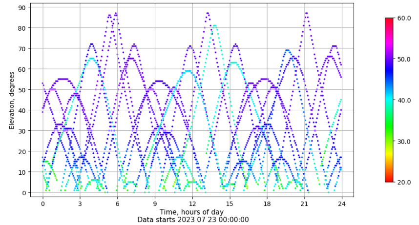
Time-elevation plot for station ZFRA. Signal to Noise S1C Data file ZFRA00ESP_R_2023204.xtr
