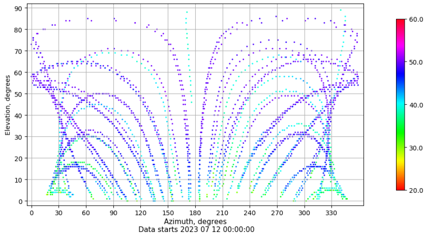
Azimuth-elevation plot for station ZFRA. Signal to Noise S1C Data file ZFRA00ESP_R_2023193.xtr
