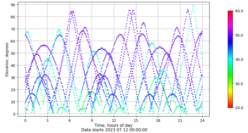
Time-elevation plot for station ZFRA. Signal to Noise S1C Data file ZFRA00ESP_R_2023193.xtr
