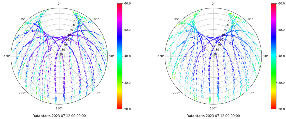
Skyplot for station ZFRA. Signal to Noise S1C Data file ZFRA00ESP_R_2023193.xtr Skyplot for station ZFRA. Signal to Noise S2P Data file ZFRA00ESP_R_2023193.xtr
