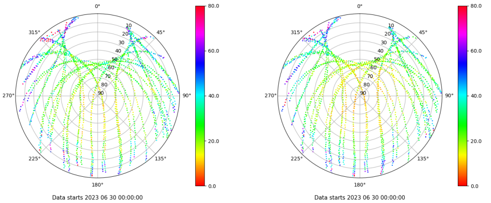
Skyplot for station ZFRA. Parameter M1C Data file ZFRA00ESP_R_2023181.xtr Skyplot for station ZFRA. Parameter M2P Data file ZFRA00ESP_R_2023181.xtr
