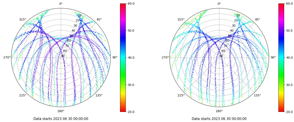
Skyplot for station ZFRA. Signal to Noise S1C Data file ZFRA00ESP_R_2023181.xtr Skyplot for station ZFRA. Signal to Noise S2P Data file ZFRA00ESP_R_2023181.xtr
