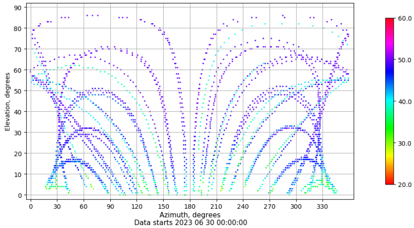
Azimuth-elevation plot for station ZFRA. Signal to Noise S1C Data file ZFRA00ESP_R_2023181.xtr
