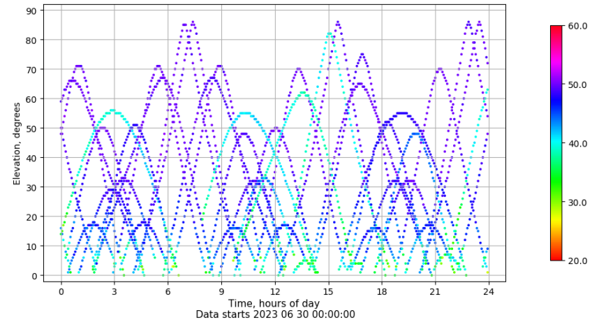
Time-elevation plot for station ZFRA. Signal to Noise S1C Data file ZFRA00ESP_R_2023181.xtr
