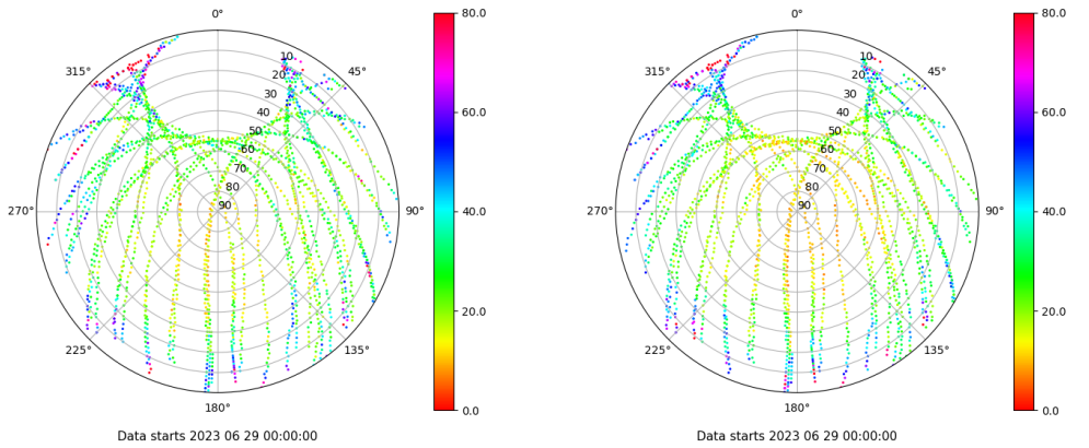
Skyplot for station ZFRA. Parameter M1C Data file ZFRA00ESP_R_2023180.xtr Skyplot for station ZFRA. Parameter M2P Data file ZFRA00ESP_R_2023180.xtr
