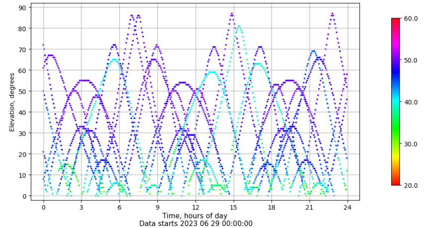
Time-elevation plot for station ZFRA. Signal to Noise S1C Data file ZFRA00ESP_R_2023180.xtr
