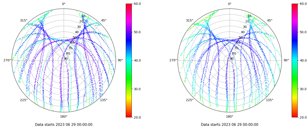
Skyplot for station ZFRA. Signal to Noise S1C Data file ZFRA00ESP_R_2023180.xtr Skyplot for station ZFRA. Signal to Noise S2P Data file ZFRA00ESP_R_2023180.xtr
