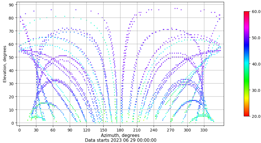
Azimuth-elevation plot for station ZFRA. Signal to Noise S1C Data file ZFRA00ESP_R_2023180.xtr
