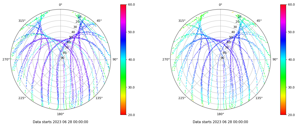
Skyplot for station ZFRA. Signal to Noise S1C Data file ZFRA00ESP_R_2023179.xtr Skyplot for station ZFRA. Signal to Noise S2P Data file ZFRA00ESP_R_2023179.xtr
