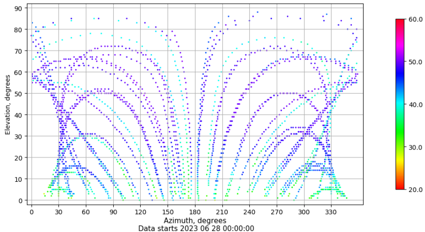
Azimuth-elevation plot for station ZFRA. Signal to Noise S1C Data file ZFRA00ESP_R_2023179.xtr
