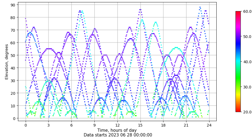
Time-elevation plot for station ZFRA. Signal to Noise S1C Data file ZFRA00ESP_R_2023179.xtr
