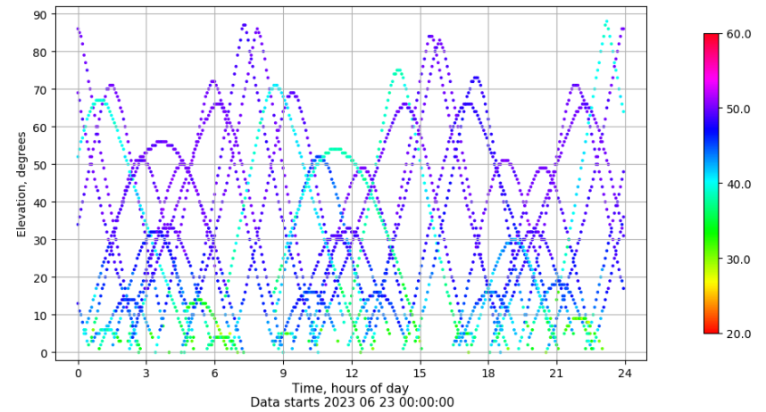
Time-elevation plot for station ZFRA. Signal to Noise S1C Data file ZFRA00ESP_R_2023174.xtr
