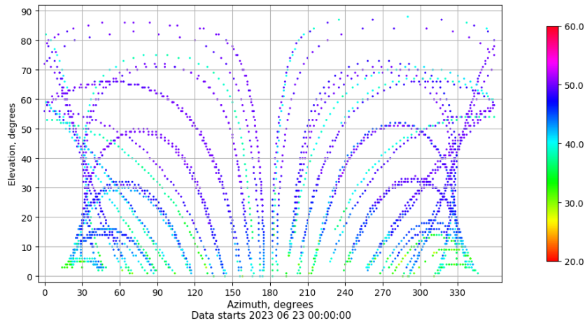
Azimuth-elevation plot for station ZFRA. Signal to Noise S1C Data file ZFRA00ESP_R_2023174.xtr
