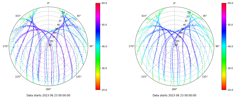
Skyplot for station ZFRA. Signal to Noise S1C Data file ZFRA00ESP_R_2023174.xtr Skyplot for station ZFRA. Signal to Noise S2P Data file ZFRA00ESP_R_2023174.xtr
