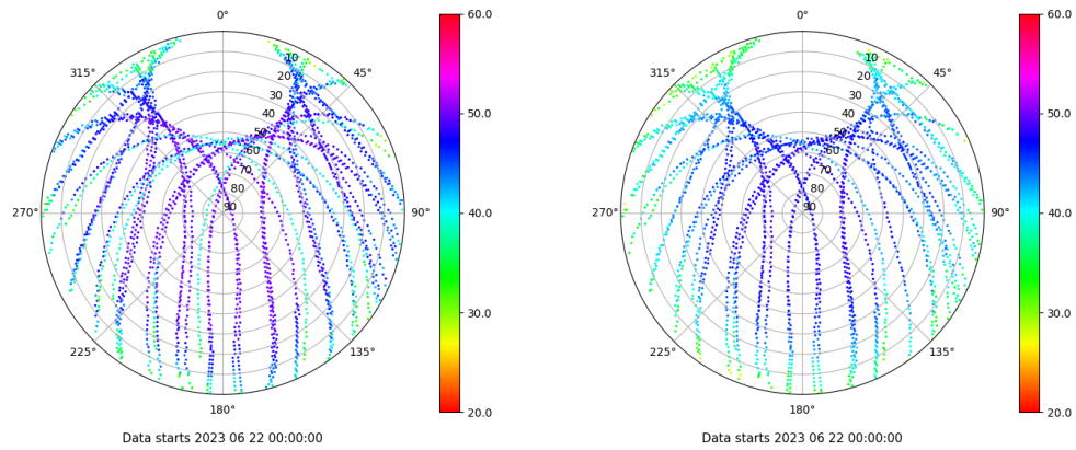
Skyplot for station ZFRA. Signal to Noise S1C Data file ZFRA00ESP_R_2023173.xtr Skyplot for station ZFRA. Signal to Noise S2P Data file ZFRA00ESP_R_2023173.xtr
