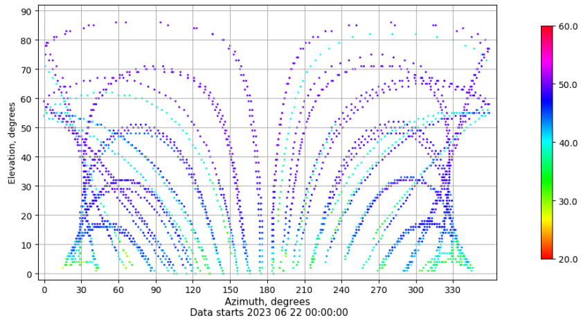
Azimuth-elevation plot for station ZFRA. Signal to Noise S1C Data file ZFRA00ESP_R_2023173.xtr
