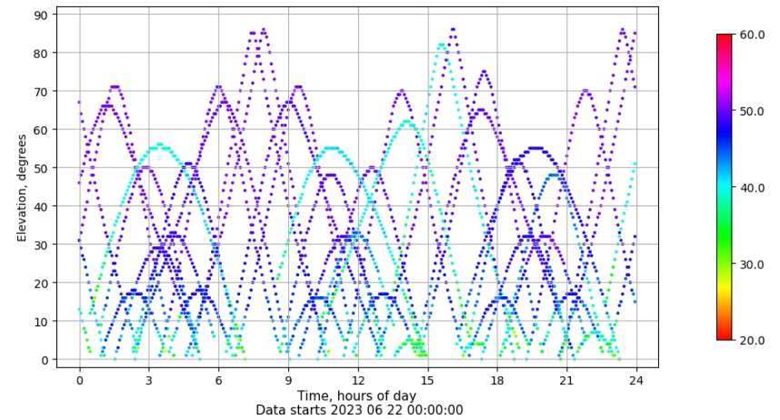
Time-elevation plot for station ZFRA. Signal to Noise S1C Data file ZFRA00ESP_R_2023173.xtr
