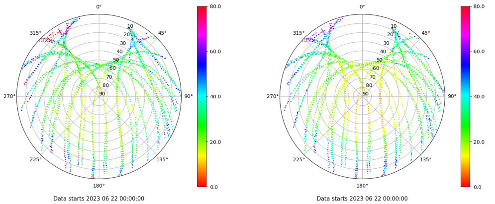
Skyplot for station ZFRA. Parameter M1C Data file ZFRA00ESP_R_2023173.xtr Skyplot for station ZFRA. Parameter M2P Data file ZFRA00ESP_R_2023173.xtr
