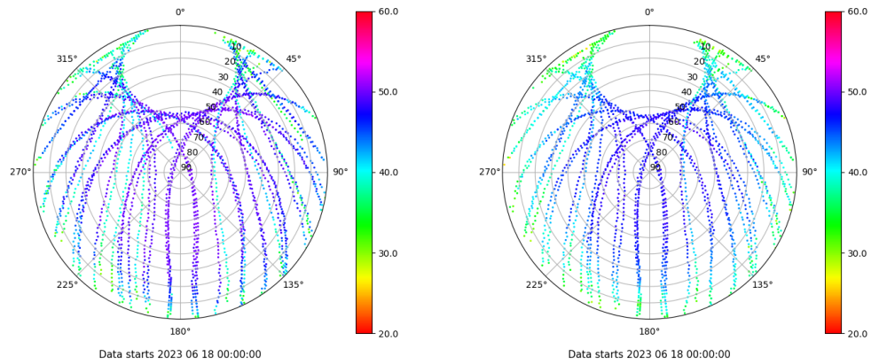
Skyplot for station ZFRA. Signal to Noise S1C Data file ZFRA00ESP_R_2023169.xtr Skyplot for station ZFRA. Signal to Noise S2P Data file ZFRA00ESP_R_2023169.xtr
