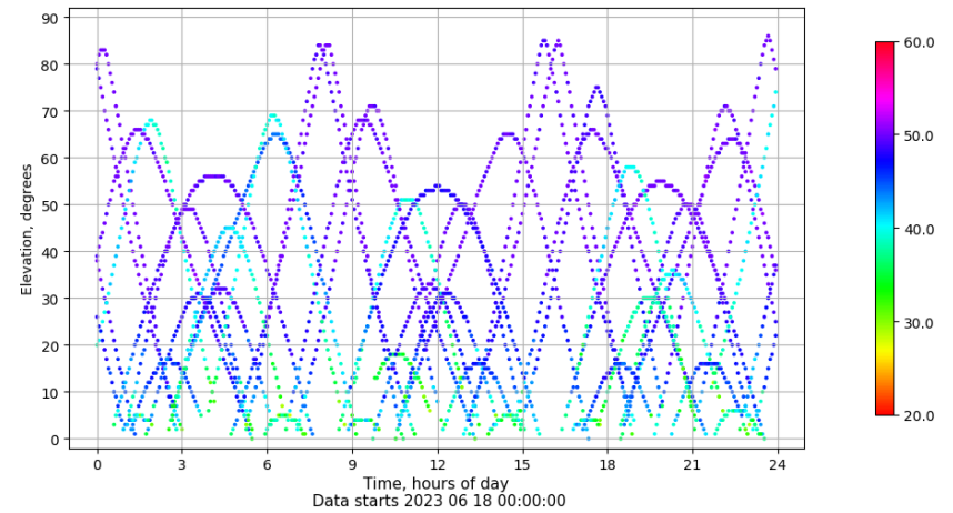
Time-elevation plot for station ZFRA. Signal to Noise S1C Data file ZFRA00ESP_R_2023169.xtr
