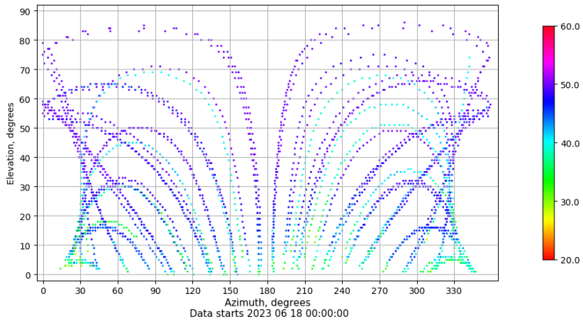
Azimuth-elevation plot for station ZFRA. Signal to Noise S1C Data file ZFRA00ESP_R_2023169.xtr
