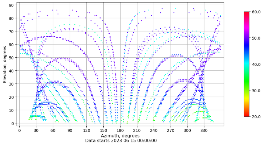
Azimuth-elevation plot for station ZFRA. Signal to Noise S1C Data file ZFRA00ESP_R_2023166.xtr
