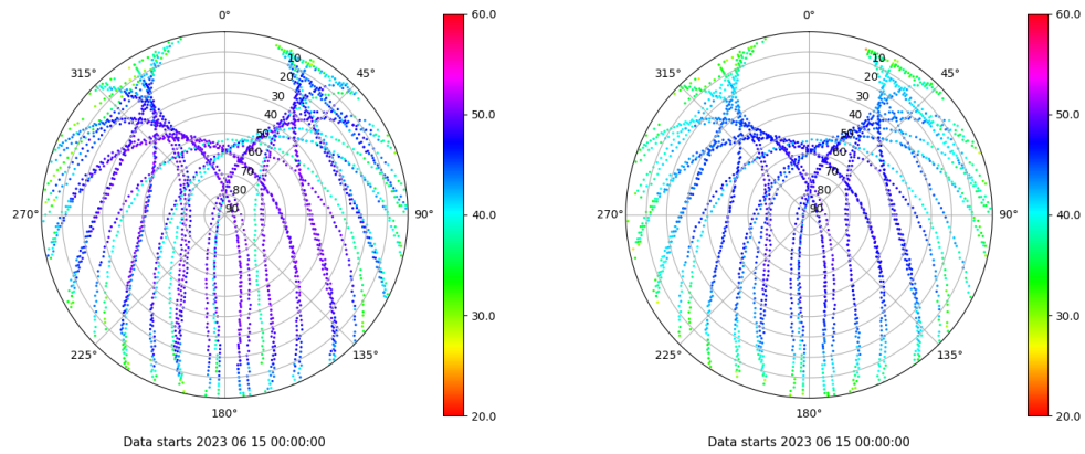
Skyplot for station ZFRA. Signal to Noise S1C Data file ZFRA00ESP_R_2023166.xtr Skyplot for station ZFRA. Signal to Noise S2P Data file ZFRA00ESP_R_2023166.xtr
