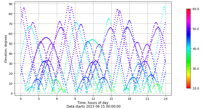
Time-elevation plot for station ZFRA. Signal to Noise S1C Data file ZFRA00ESP_R_2023166.xtr
