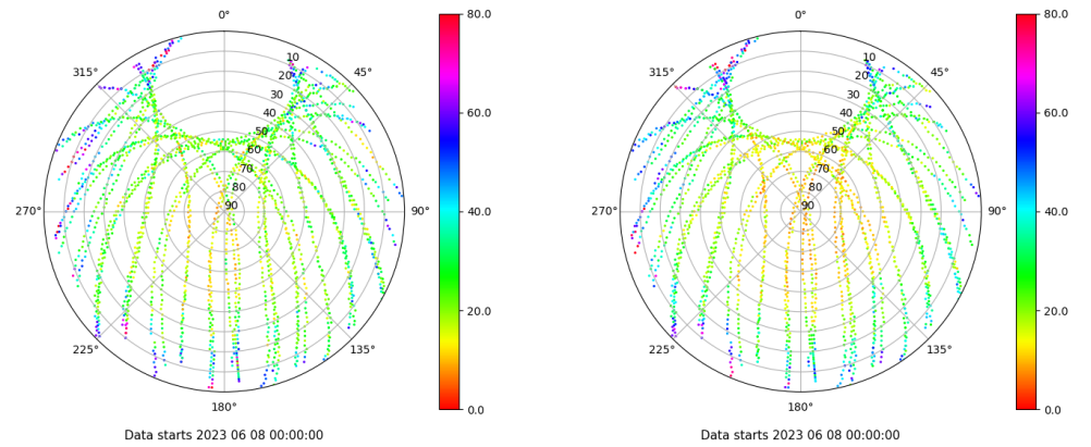
Skyplot for station ZFRA. Parameter M1C Data file ZFRA00ESP_R_2023159.xtr Skyplot for station ZFRA. Parameter M2P Data file ZFRA00ESP_R_2023159.xtr
