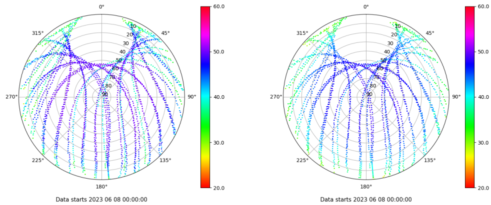
Skyplot for station ZFRA. Signal to Noise S1C Data file ZFRA00ESP_R_2023159.xtr Skyplot for station ZFRA. Signal to Noise S2P Data file ZFRA00ESP_R_2023159.xtr
