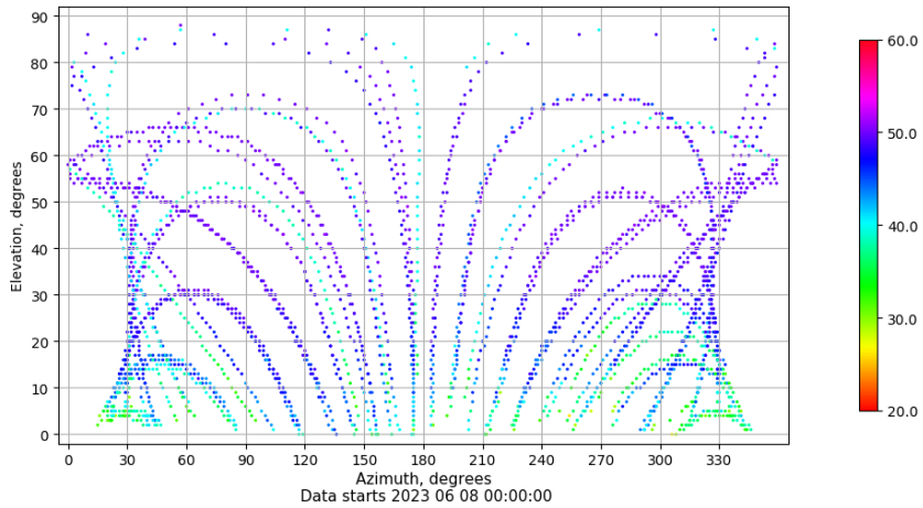
Azimuth-elevation plot for station ZFRA. Signal to Noise S1C Data file ZFRA00ESP_R_2023159.xtr
