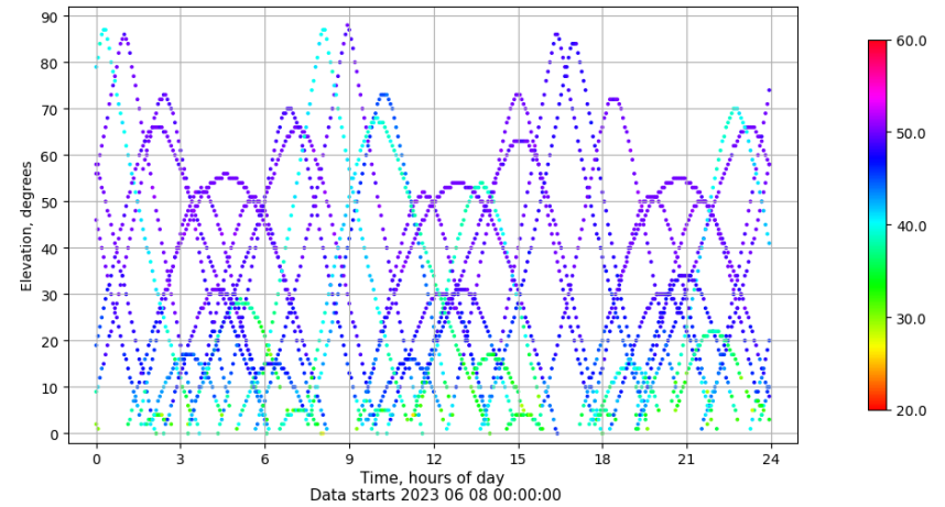
Time-elevation plot for station ZFRA. Signal to Noise S1C Data file ZFRA00ESP_R_2023159.xtr
