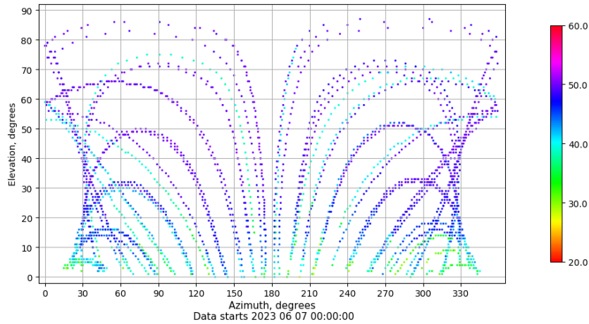
Azimuth-elevation plot for station ZFRA. Signal to Noise S1C Data file ZFRA00ESP_R_2023158.xtr
