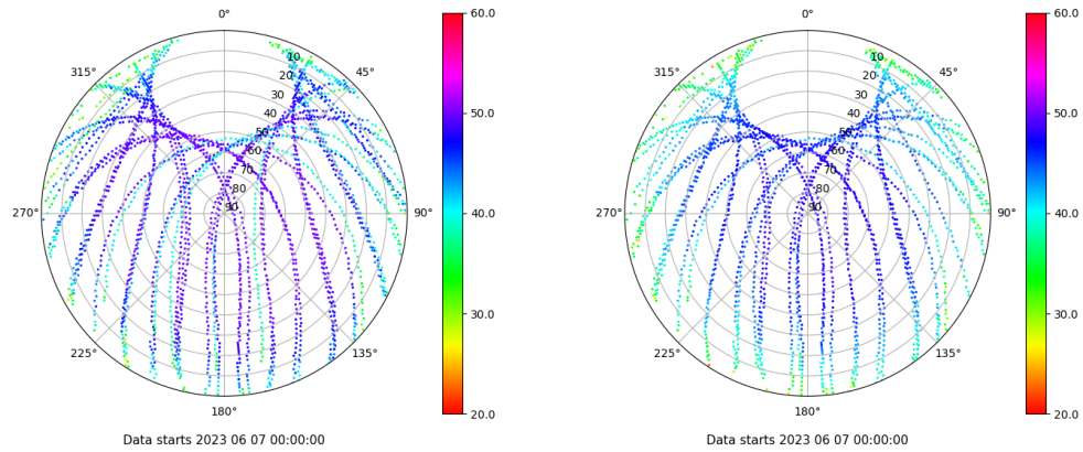
Skyplot for station ZFRA. Signal to Noise S1C Data file ZFRA00ESP_R_2023158.xtr Skyplot for station ZFRA. Signal to Noise S2P Data file ZFRA00ESP_R_2023158.xtr
