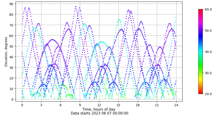
Time-elevation plot for station ZFRA. Signal to Noise S1C Data file ZFRA00ESP_R_2023158.xtr
