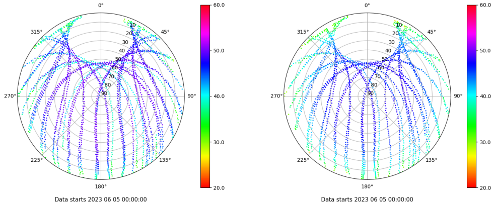
Skyplot for station ZFRA. Signal to Noise S1C Data file ZFRA00ESP_R_2023156.xtr Skyplot for station ZFRA. Signal to Noise S2P Data file ZFRA00ESP_R_2023156.xtr
