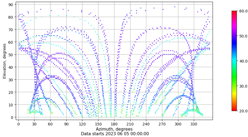
Azimuth-elevation plot for station ZFRA. Signal to Noise S1C Data file ZFRA00ESP_R_2023156.xtr
