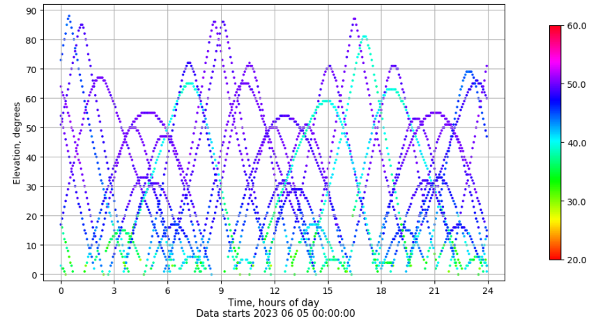
Time-elevation plot for station ZFRA. Signal to Noise S1C Data file ZFRA00ESP_R_2023156.xtr
