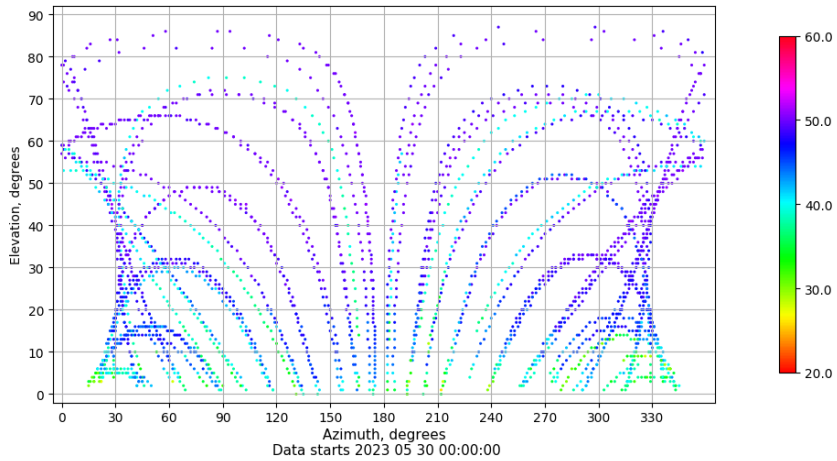
Azimuth-elevation plot for station ZFRA. Signal to Noise S1C Data file ZFRA00ESP_R_2023150.xtr
