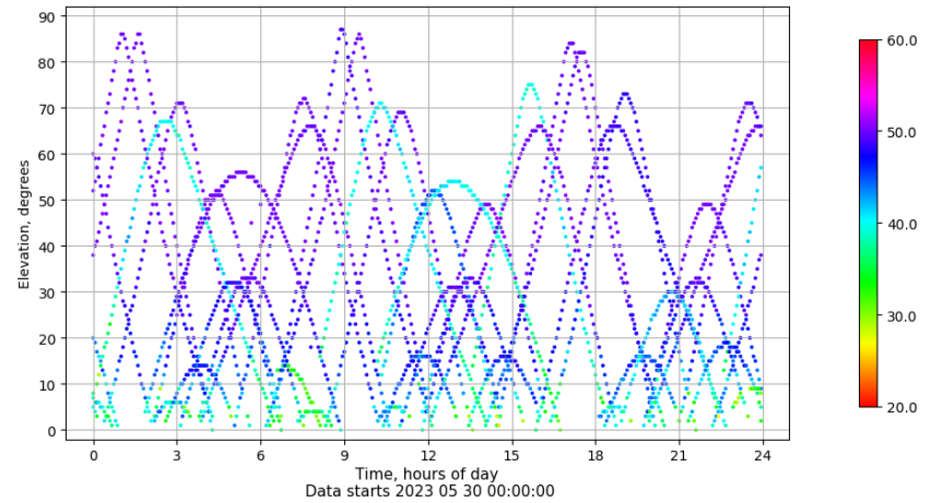
Time-elevation plot for station ZFRA. Signal to Noise S1C Data file ZFRA00ESP_R_2023150.xtr
