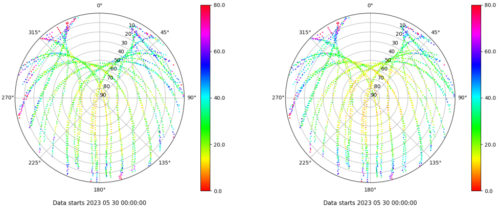
Skyplot for station ZFRA. Parameter M1C Data file ZFRA00ESP_R_2023150.xtr Skyplot for station ZFRA. Parameter M2P Data file ZFRA00ESP_R_2023150.xtr
