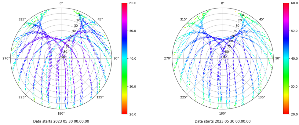
Skyplot for station ZFRA. Signal to Noise S1C Data file ZFRA00ESP_R_2023150.xtr Skyplot for station ZFRA. Signal to Noise S2P Data file ZFRA00ESP_R_2023150.xtr
