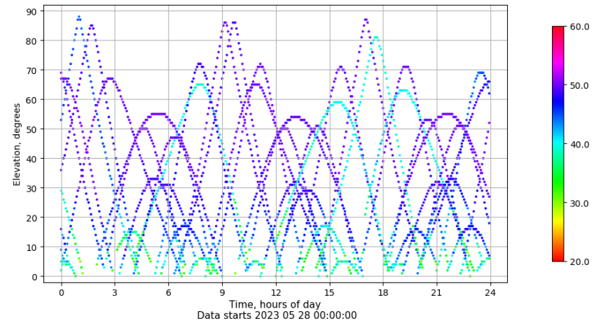
Time-elevation plot for station ZFRA. Signal to Noise S1C Data file ZFRA00ESP_R_2023148.xtr
