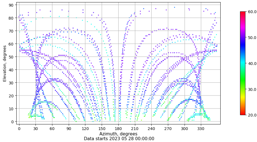
Azimuth-elevation plot for station ZFRA. Signal to Noise S1C Data file ZFRA00ESP_R_2023148.xtr
