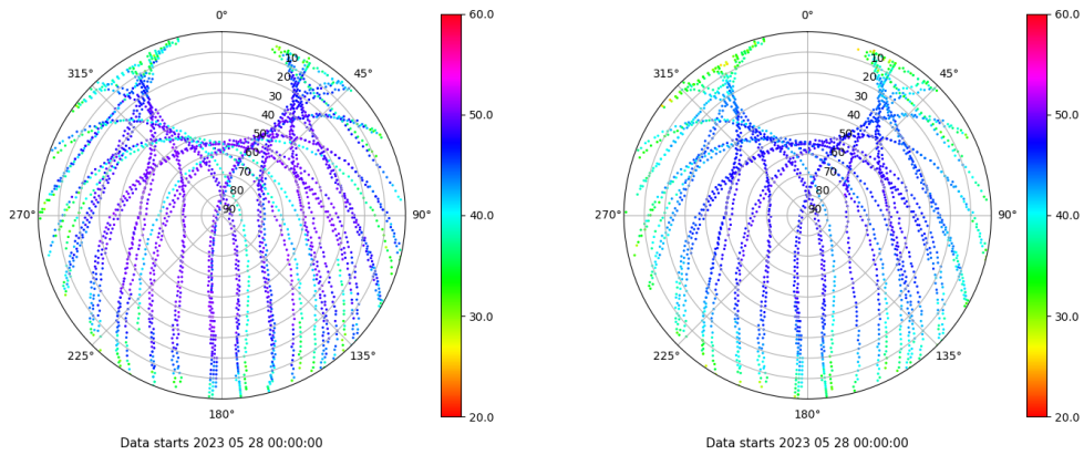
Skyplot for station ZFRA. Signal to Noise S1C Data file ZFRA00ESP_R_2023148.xtr Skyplot for station ZFRA. Signal to Noise S2P Data file ZFRA00ESP_R_2023148.xtr
