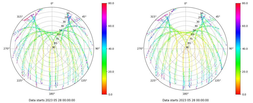
Skyplot for station ZFRA. Parameter M1C Data file ZFRA00ESP_R_2023148.xtr Skyplot for station ZFRA. Parameter M2P Data file ZFRA00ESP_R_2023148.xtr
