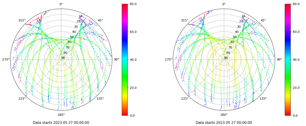
Skyplot for station ZFRA. Parameter M1C Data file ZFRA00ESP_R_2023147.xtr Skyplot for station ZFRA. Parameter M2P Data file ZFRA00ESP_R_2023147.xtr
