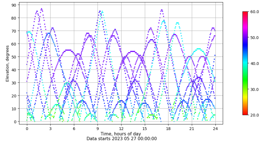
Time-elevation plot for station ZFRA. Signal to Noise S1C Data file ZFRA00ESP_R_2023147.xtr
