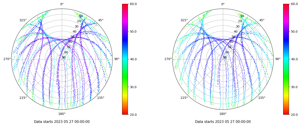
Skyplot for station ZFRA. Signal to Noise S1C Data file ZFRA00ESP_R_2023147.xtr Skyplot for station ZFRA. Signal to Noise S2P Data file ZFRA00ESP_R_2023147.xtr
