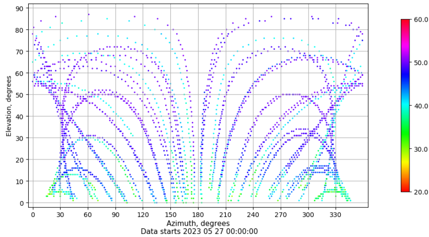
Azimuth-elevation plot for station ZFRA. Signal to Noise S1C Data file ZFRA00ESP_R_2023147.xtr
