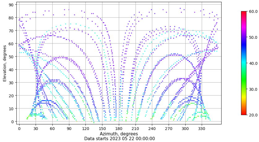
Azimuth-elevation plot for station ZFRA. Signal to Noise S1C Data file ZFRA00ESP_R_2023142.xtr
