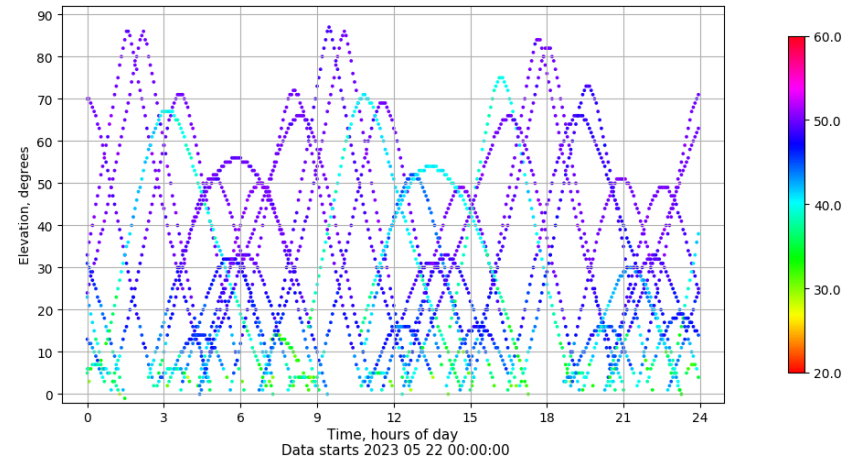
Time-elevation plot for station ZFRA. Signal to Noise S1C Data file ZFRA00ESP_R_2023142.xtr
