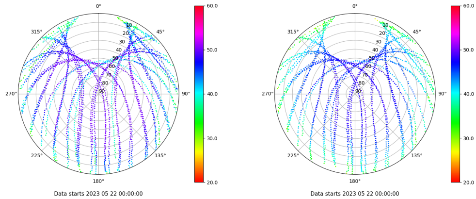
Skyplot for station ZFRA. Signal to Noise S1C Data file ZFRA00ESP_R_2023142.xtr Skyplot for station ZFRA. Signal to Noise S2P Data file ZFRA00ESP_R_2023142.xtr
