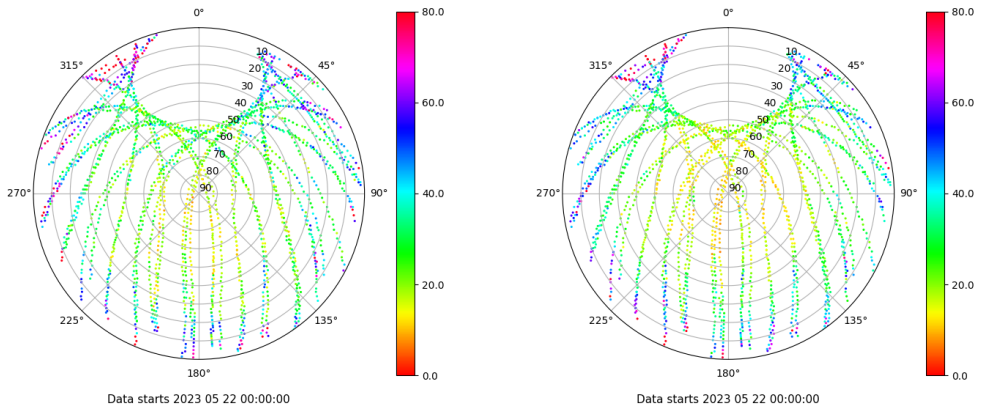
Skyplot for station ZFRA. Parameter M1C Data file ZFRA00ESP_R_2023142.xtr Skyplot for station ZFRA. Parameter M2P Data file ZFRA00ESP_R_2023142.xtr
