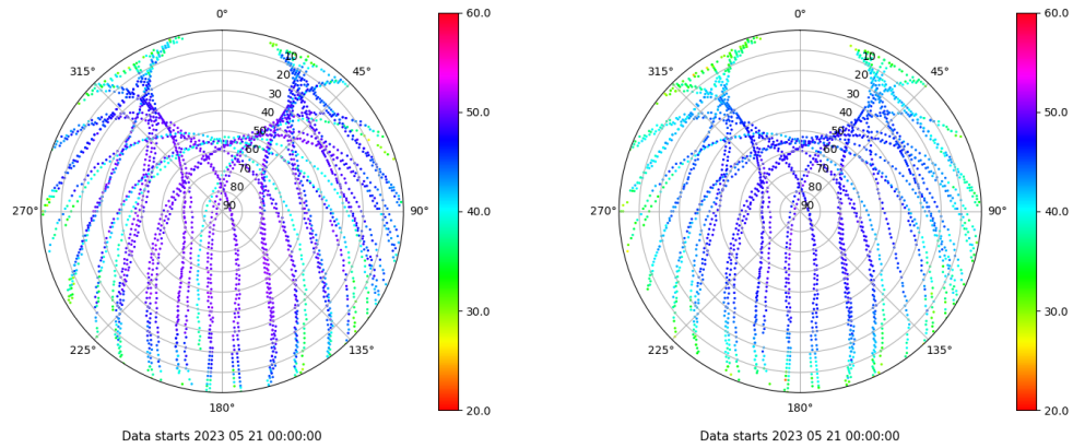
Skyplot for station ZFRA. Signal to Noise S1C Data file ZFRA00ESP_R_2023141.xtr Skyplot for station ZFRA. Signal to Noise S2P Data file ZFRA00ESP_R_2023141.xtr
