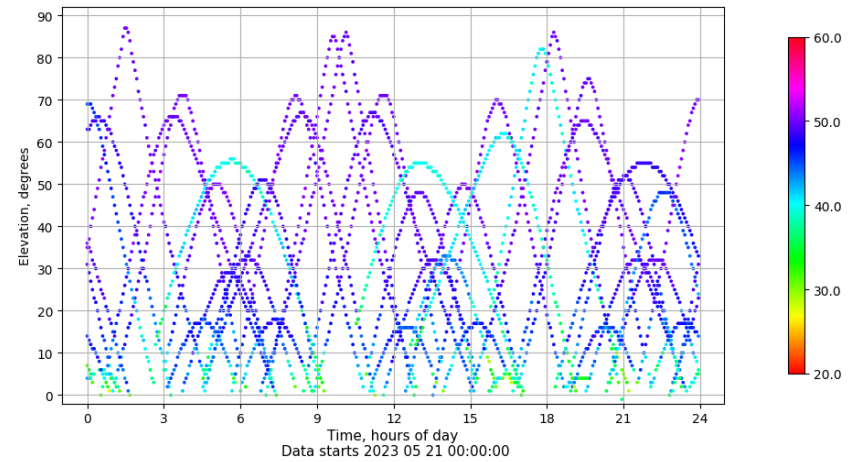
Time-elevation plot for station ZFRA. Signal to Noise S1C Data file ZFRA00ESP_R_2023141.xtr
