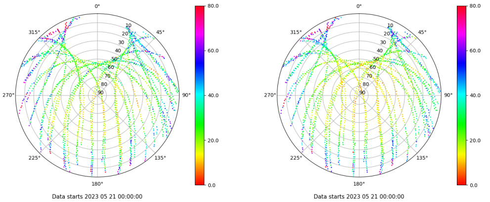
Skyplot for station ZFRA. Parameter M1C Data file ZFRA00ESP_R_2023141.xtr Skyplot for station ZFRA. Parameter M2P Data file ZFRA00ESP_R_2023141.xtr
