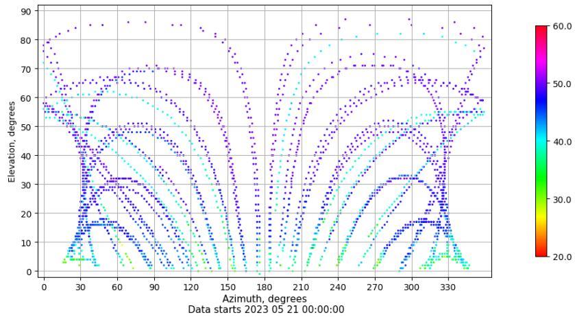
Azimuth-elevation plot for station ZFRA. Signal to Noise S1C Data file ZFRA00ESP_R_2023141.xtr
