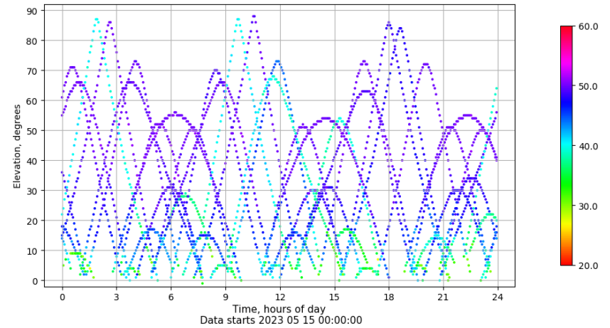
Time-elevation plot for station ZFRA. Signal to Noise S1C Data file ZFRA00ESP_R_2023135.xtr
