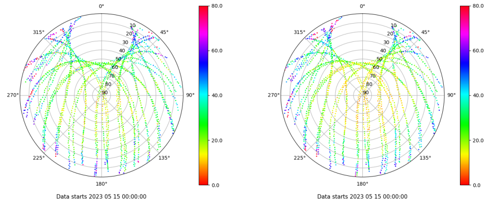
Skyplot for station ZFRA. Parameter M1C Data file ZFRA00ESP_R_2023135.xtr Skyplot for station ZFRA. Parameter M2P Data file ZFRA00ESP_R_2023135.xtr
