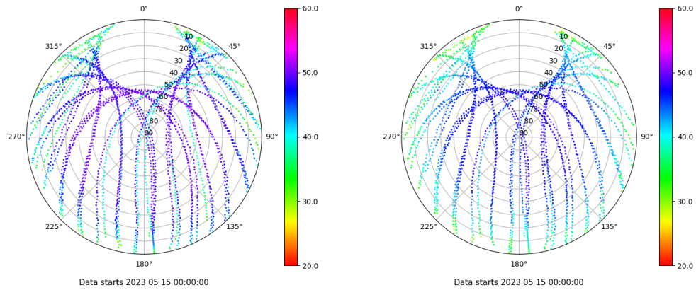
Skyplot for station ZFRA. Signal to Noise S1C Data file ZFRA00ESP_R_2023135.xtr Skyplot for station ZFRA. Signal to Noise S2P Data file ZFRA00ESP_R_2023135.xtr
