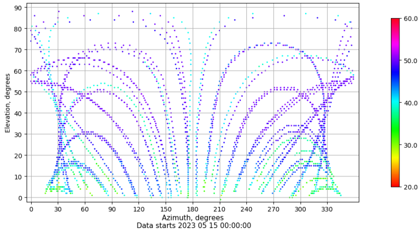
Azimuth-elevation plot for station ZFRA. Signal to Noise S1C Data file ZFRA00ESP_R_2023135.xtr
