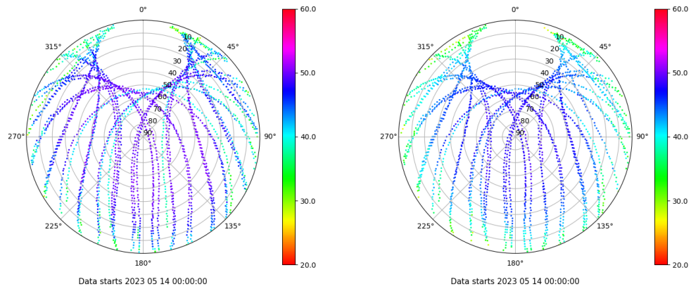
Skyplot for station ZFRA. Signal to Noise S1C Data file ZFRA00ESP_R_2023134.xtr Skyplot for station ZFRA. Signal to Noise S2P Data file ZFRA00ESP_R_2023134.xtr
