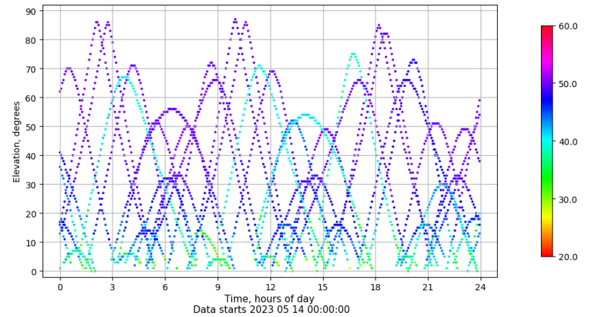
Time-elevation plot for station ZFRA. Signal to Noise S1C Data file ZFRA00ESP_R_2023134.xtr
