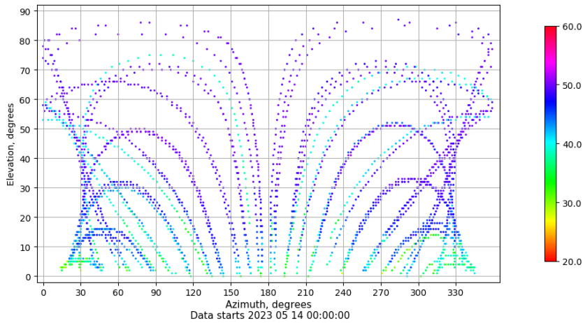
Azimuth-elevation plot for station ZFRA. Signal to Noise S1C Data file ZFRA00ESP_R_2023134.xtr
