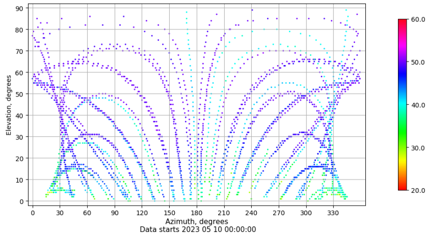
Azimuth-elevation plot for station ZFRA. Signal to Noise S1C Data file ZFRA00ESP_R_2023130.xtr
