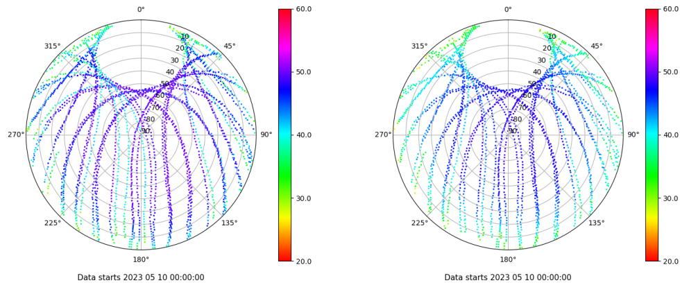
Skyplot for station ZFRA. Signal to Noise S1C Data file ZFRA00ESP_R_2023130.xtr Skyplot for station ZFRA. Signal to Noise S2P Data file ZFRA00ESP_R_2023130.xtr
