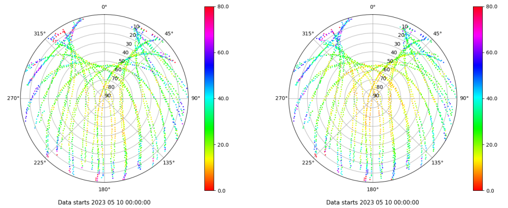
Skyplot for station ZFRA. Parameter M1C Data file ZFRA00ESP_R_2023130.xtr Skyplot for station ZFRA. Parameter M2P Data file ZFRA00ESP_R_2023130.xtr
