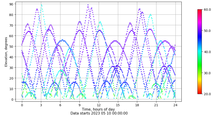
Time-elevation plot for station ZFRA. Signal to Noise S1C Data file ZFRA00ESP_R_2023130.xtr
