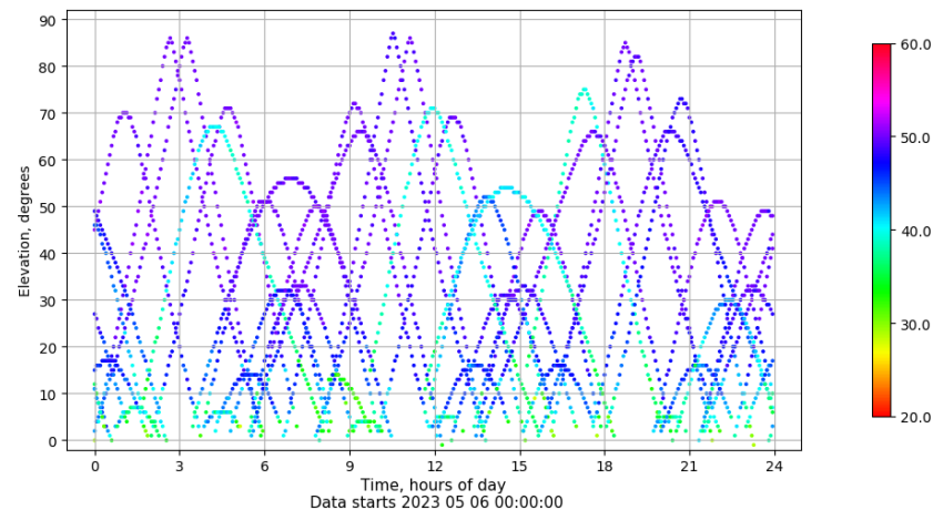
Time-elevation plot for station ZFRA. Signal to Noise S1C Data file ZFRA00ESP_R_2023126.xtr
