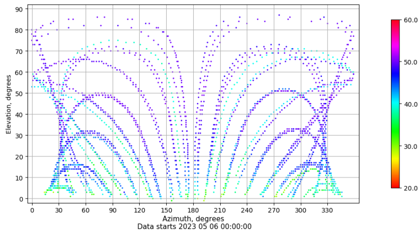
Azimuth-elevation plot for station ZFRA. Signal to Noise S1C Data file ZFRA00ESP_R_2023126.xtr
