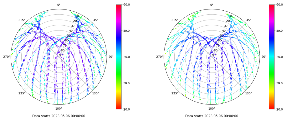
Skyplot for station ZFRA. Signal to Noise S1C Data file ZFRA00ESP_R_2023126.xtr Skyplot for station ZFRA. Signal to Noise S2P Data file ZFRA00ESP_R_2023126.xtr
