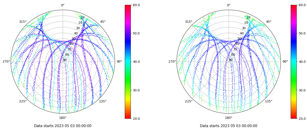
Skyplot for station ZFRA. Signal to Noise S1C Data file ZFRA00ESP_R_2023123.xtr Skyplot for station ZFRA. Signal to Noise S2P Data file ZFRA00ESP_R_2023123.xtr
