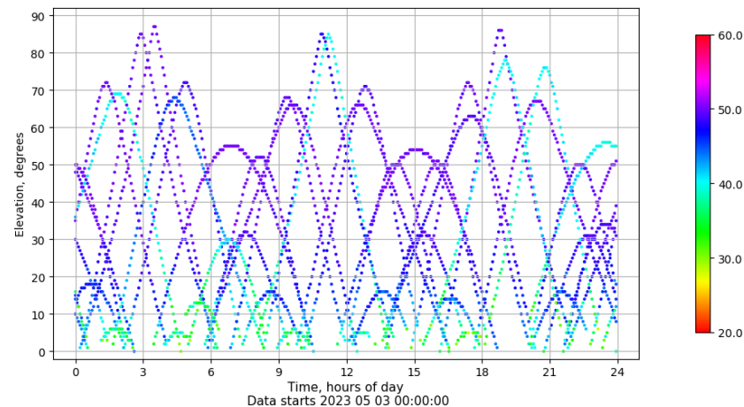
Time-elevation plot for station ZFRA. Signal to Noise S1C Data file ZFRA00ESP_R_2023123.xtr
