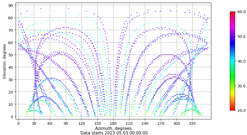
Azimuth-elevation plot for station ZFRA. Signal to Noise S1C Data file ZFRA00ESP_R_2023123.xtr
