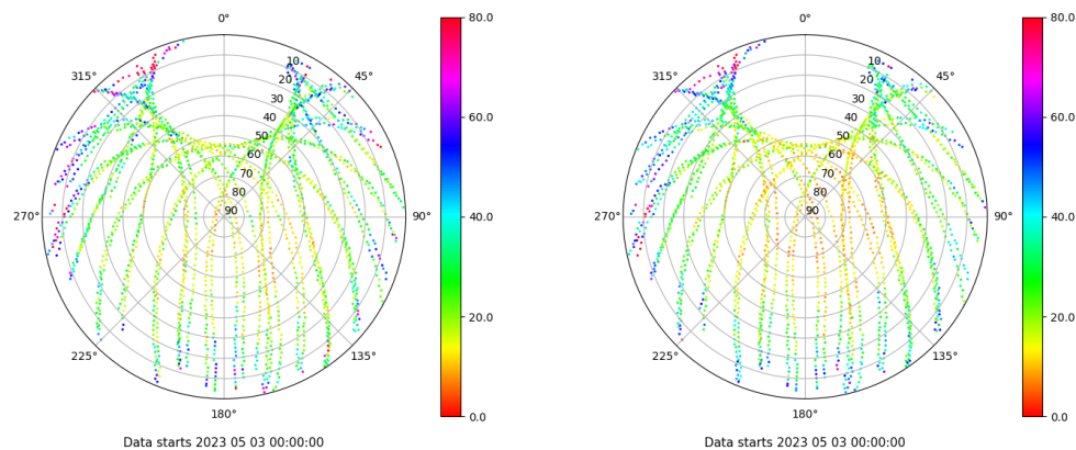
Skyplot for station ZFRA. Parameter M1C Data file ZFRA00ESP_R_2023123.xtr Skyplot for station ZFRA. Parameter M2P Data file ZFRA00ESP_R_2023123.xtr
