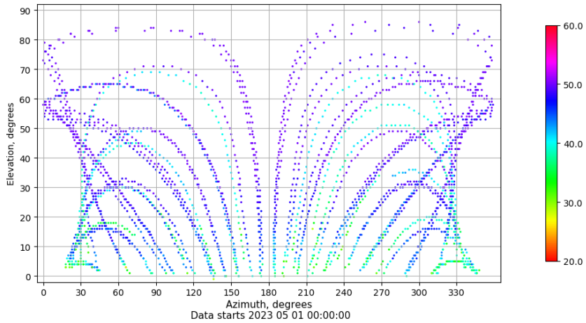
Azimuth-elevation plot for station ZFRA. Signal to Noise S1C Data file ZFRA00ESP_R_2023121.xtr
