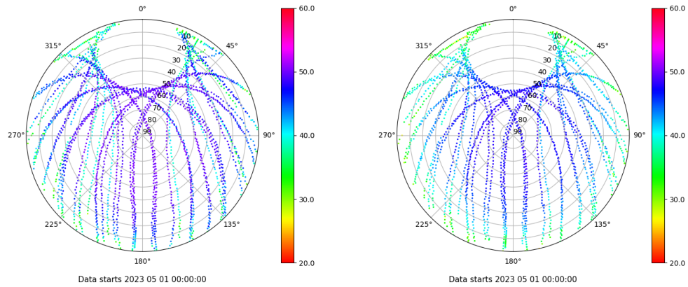
Skyplot for station ZFRA. Signal to Noise S1C Data file ZFRA00ESP_R_2023121.xtr Skyplot for station ZFRA. Signal to Noise S2P Data file ZFRA00ESP_R_2023121.xtr
