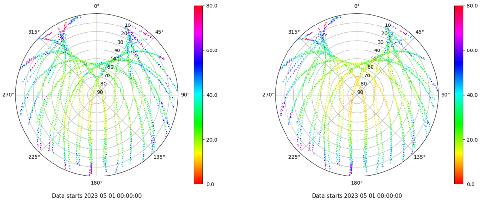
Skyplot for station ZFRA. Parameter M1C Data file ZFRA00ESP_R_2023121.xtr Skyplot for station ZFRA. Parameter M2P Data file ZFRA00ESP_R_2023121.xtr
