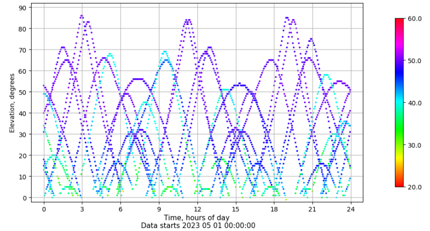
Time-elevation plot for station ZFRA. Signal to Noise S1C Data file ZFRA00ESP_R_2023121.xtr
