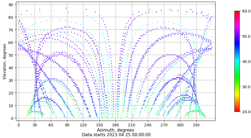
Azimuth-elevation plot for station ZFRA. Signal to Noise S1C Data file ZFRA00ESP_R_2023115.xtr
