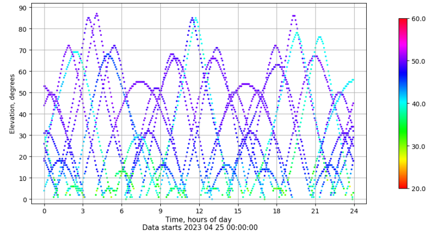
Time-elevation plot for station ZFRA. Signal to Noise S1C Data file ZFRA00ESP_R_2023115.xtr
