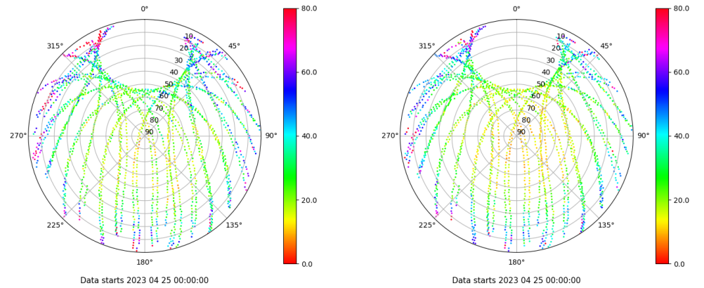
Skyplot for station ZFRA. Parameter M1C Data file ZFRA00ESP_R_2023115.xtr Skyplot for station ZFRA. Parameter M2P Data file ZFRA00ESP_R_2023115.xtr
