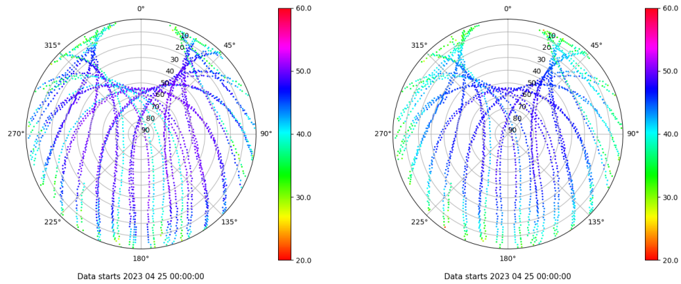
Skyplot for station ZFRA. Signal to Noise S1C Data file ZFRA00ESP_R_2023115.xtr Skyplot for station ZFRA. Signal to Noise S2P Data file ZFRA00ESP_R_2023115.xtr
