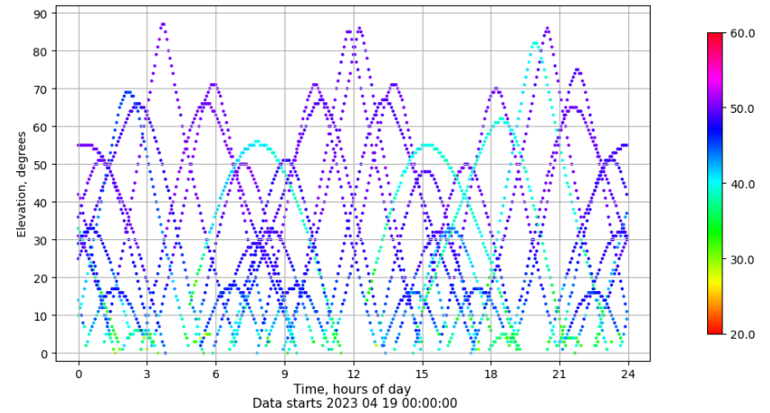
Time-elevation plot for station ZFRA. Signal to Noise S1C Data file ZFRA00ESP_R_2023109.xtr
