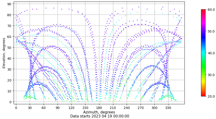
Azimuth-elevation plot for station ZFRA. Signal to Noise S1C Data file ZFRA00ESP_R_2023109.xtr
