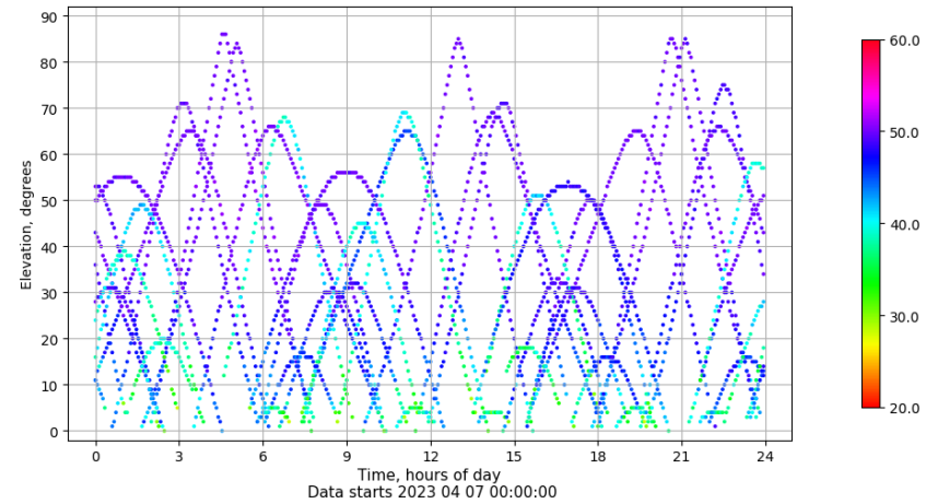
Time-elevation plot for station ZFRA. Signal to Noise S1C Data file ZFRA00ESP_R_2023097.xtr
