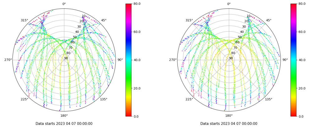
Skyplot for station ZFRA. Parameter M1C Data file ZFRA00ESP_R_2023097.xtr Skyplot for station ZFRA. Parameter M2P Data file ZFRA00ESP_R_2023097.xtr
