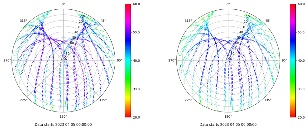
Skyplot for station ZFRA. Signal to Noise S1C Data file ZFRA00ESP_R_2023095.xtr Skyplot for station ZFRA. Signal to Noise S2P Data file ZFRA00ESP_R_2023095.xtr
