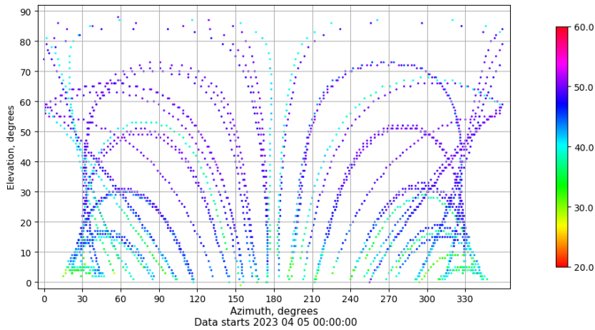
Azimuth-elevation plot for station ZFRA. Signal to Noise S1C Data file ZFRA00ESP_R_2023095.xtr
