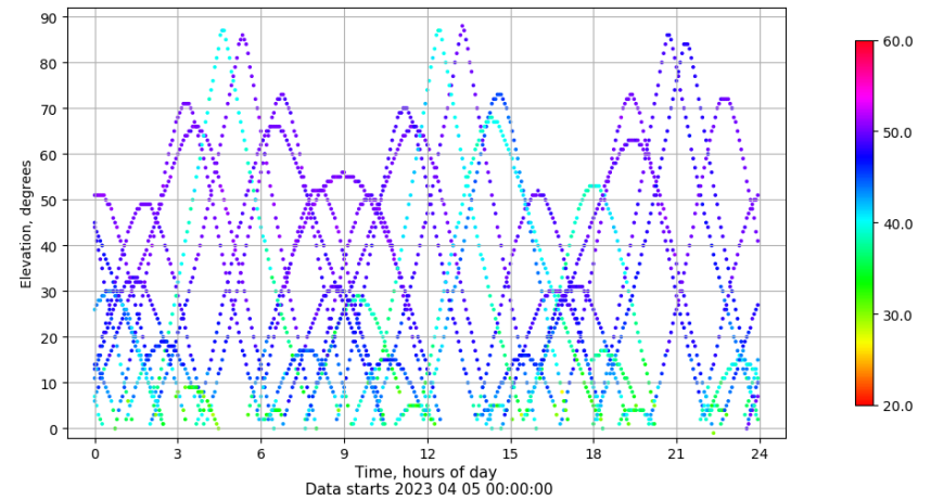
Time-elevation plot for station ZFRA. Signal to Noise S1C Data file ZFRA00ESP_R_2023095.xtr
