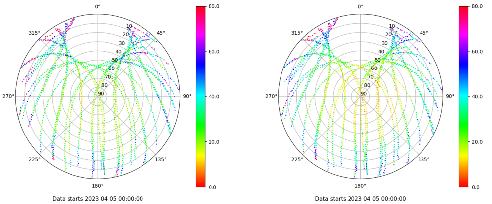
Skyplot for station ZFRA. Parameter M1C Data file ZFRA00ESP_R_2023095.xtr Skyplot for station ZFRA. Parameter M2P Data file ZFRA00ESP_R_2023095.xtr
