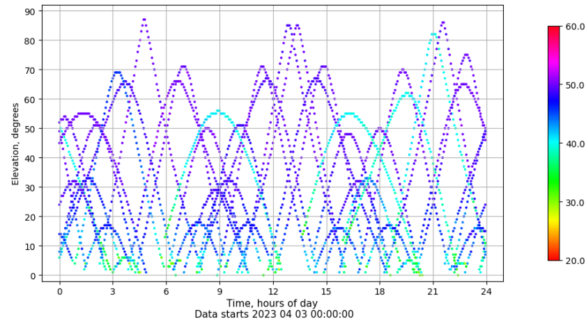
Time-elevation plot for station ZFRA. Signal to Noise S1C Data file ZFRA00ESP_R_2023093.xtr
