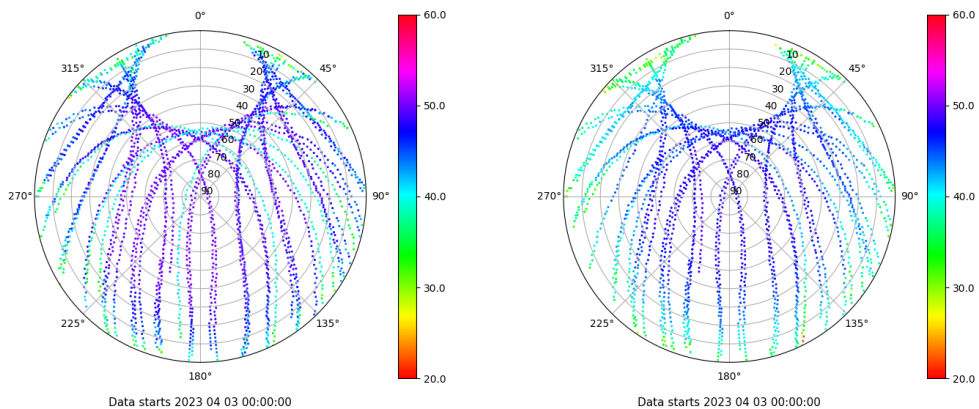
Skyplot for station ZFRA. Signal to Noise S1C Data file ZFRA00ESP_R_2023093.xtr Skyplot for station ZFRA. Signal to Noise S2P Data file ZFRA00ESP_R_2023093.xtr
