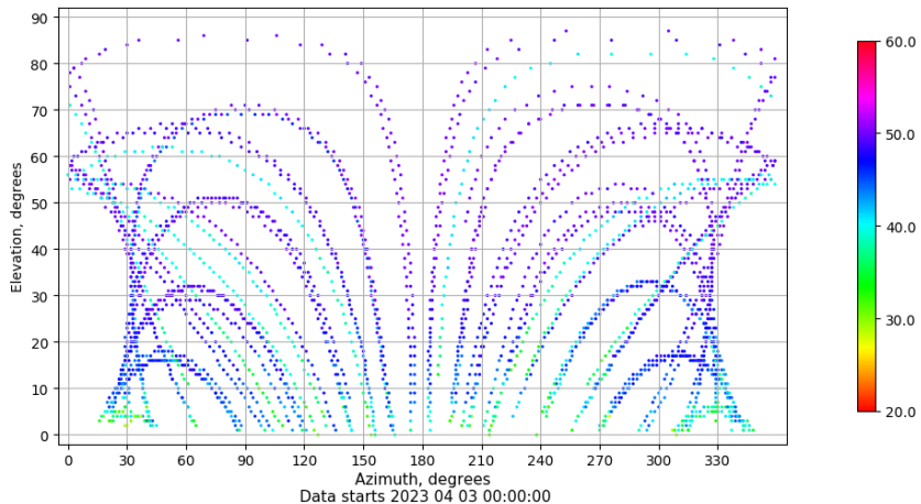
Azimuth-elevation plot for station ZFRA. Signal to Noise S1C Data file ZFRA00ESP_R_2023093.xtr
