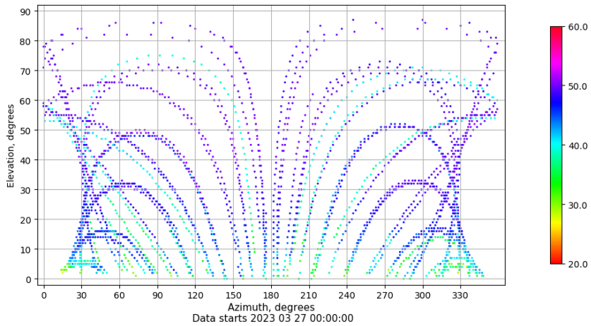
Azimuth-elevation plot for station ZFRA. Signal to Noise S1C Data file ZFRA00ESP_R_2023086.xtr
