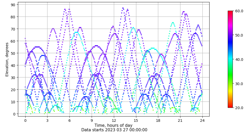
Time-elevation plot for station ZFRA. Signal to Noise S1C Data file ZFRA00ESP_R_2023086.xtr
