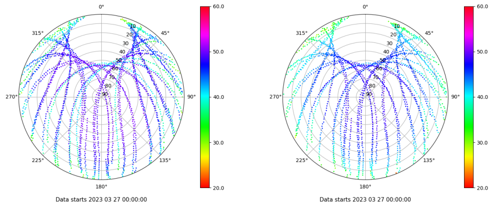
Skyplot for station ZFRA. Signal to Noise S1C Data file ZFRA00ESP_R_2023086.xtr Skyplot for station ZFRA. Signal to Noise S2P Data file ZFRA00ESP_R_2023086.xtr
