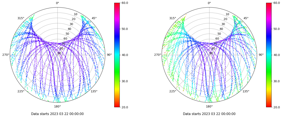
Skyplot for station ZFRA. Signal to Noise S1C Data file ZFRA00ESP_R_2023081.xtr Skyplot for station ZFRA. Signal to Noise S2W Data file ZFRA00ESP_R_2023081.xtr
