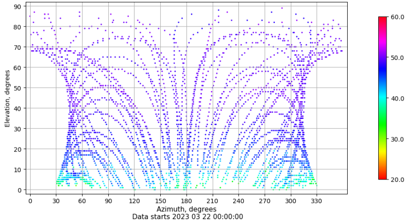
Azimuth-elevation plot for station ZFRA. Signal to Noise S1C Data file ZFRA00ESP_R_2023081.xtr
