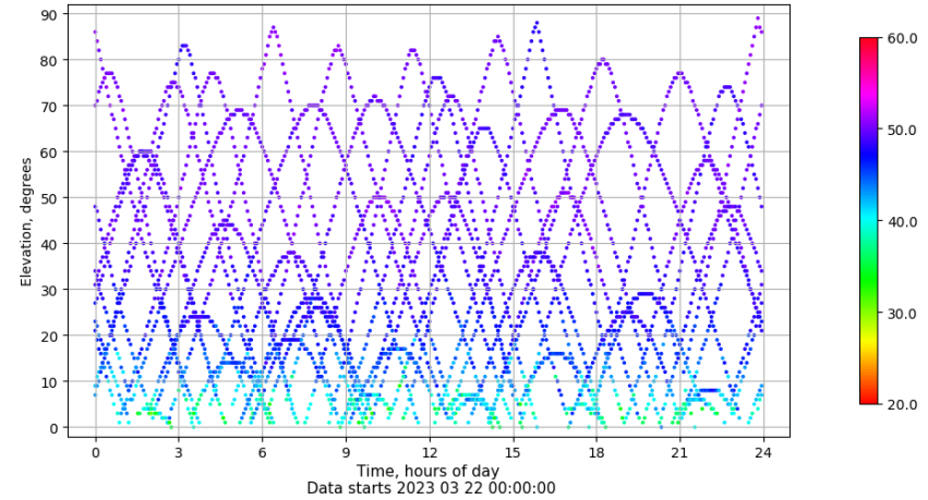
Time-elevation plot for station ZFRA. Signal to Noise S1C Data file ZFRA00ESP_R_2023081.xtr
