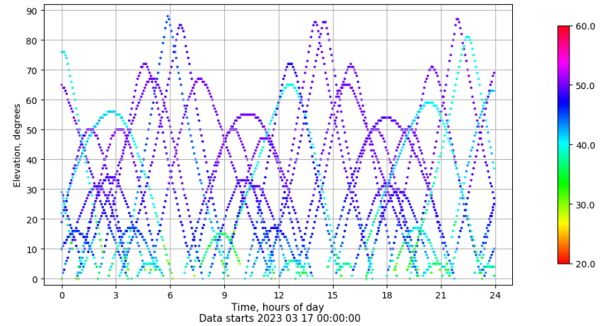
Time-elevation plot for station ZFRA. Signal to Noise S1C Data file ZFRA00ESP_R_2023076.xtr
