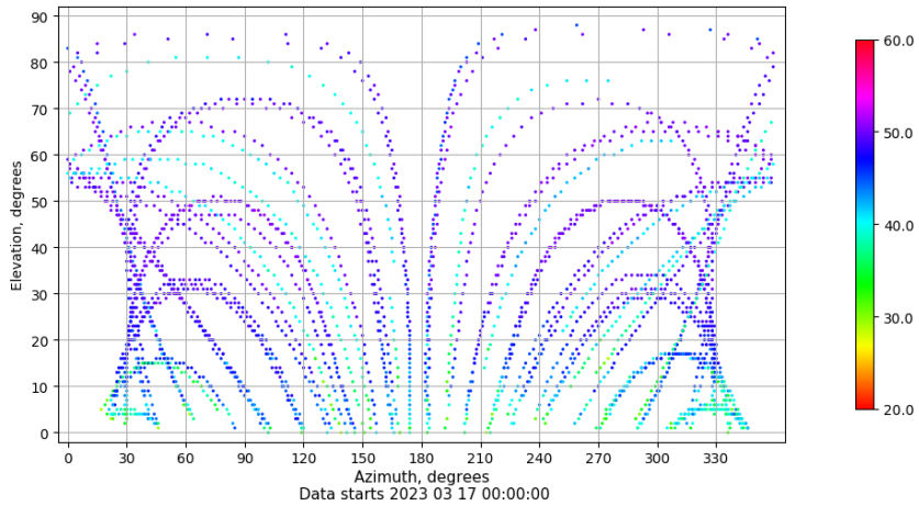
Azimuth-elevation plot for station ZFRA. Signal to Noise S1C Data file ZFRA00ESP_R_2023076.xtr
