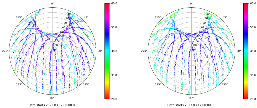
Skyplot for station ZFRA. Signal to Noise S1C Data file ZFRA00ESP_R_2023076.xtr Skyplot for station ZFRA. Signal to Noise S2P Data file ZFRA00ESP_R_2023076.xtr
