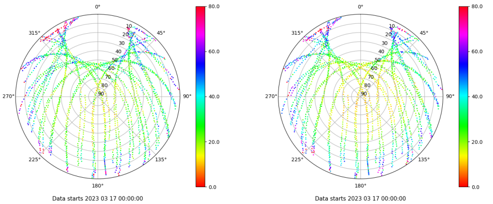
Skyplot for station ZFRA. Parameter M1C Data file ZFRA00ESP_R_2023076.xtr Skyplot for station ZFRA. Parameter M2P Data file ZFRA00ESP_R_2023076.xtr
