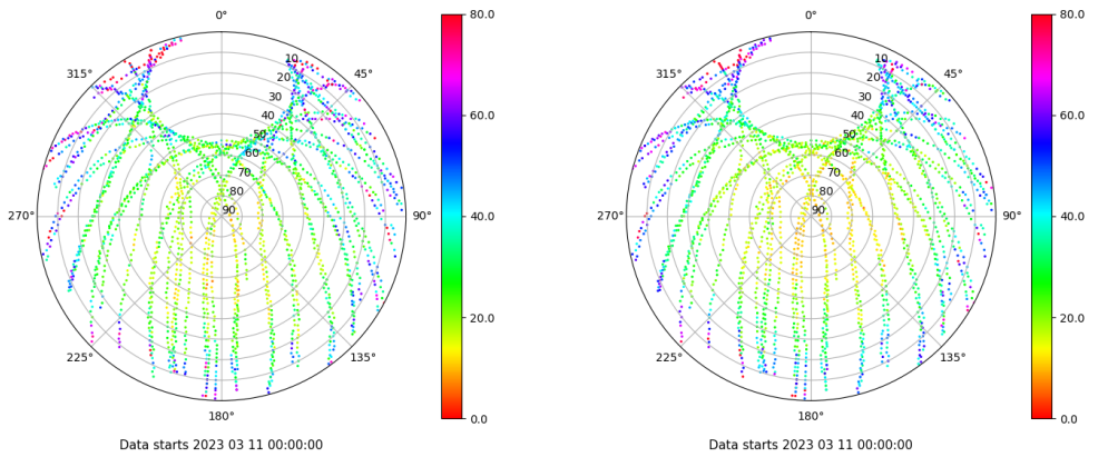
Skyplot for station ZFRA. Parameter M1C Data file ZFRA00ESP_R_2023070.xtr Skyplot for station ZFRA. Parameter M2P Data file ZFRA00ESP_R_2023070.xtr
