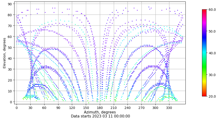
Azimuth-elevation plot for station ZFRA. Signal to Noise S1C Data file ZFRA00ESP_R_2023070.xtr
