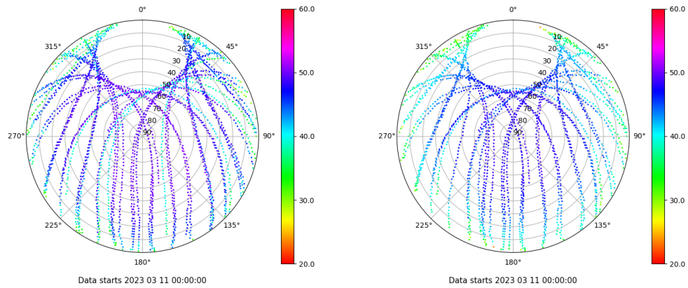
Skyplot for station ZFRA. Signal to Noise S1C Data file ZFRA00ESP_R_2023070.xtr Skyplot for station ZFRA. Signal to Noise S2P Data file ZFRA00ESP_R_2023070.xtr
