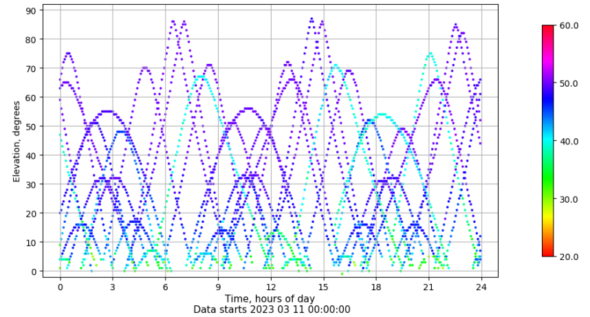
Time-elevation plot for station ZFRA. Signal to Noise S1C Data file ZFRA00ESP_R_2023070.xtr
