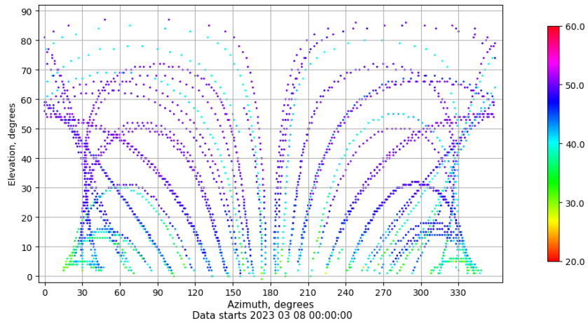
Azimuth-elevation plot for station ZFRA. Signal to Noise S1C Data file ZFRA00ESP_R_2023067.xtr
