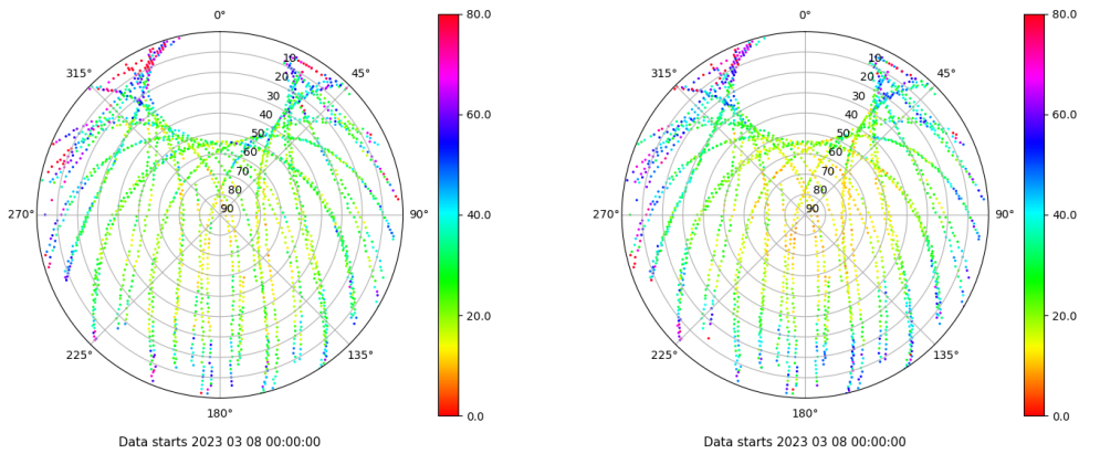
Skyplot for station ZFRA. Parameter M1C Data file ZFRA00ESP_R_2023067.xtr Skyplot for station ZFRA. Parameter M2P Data file ZFRA00ESP_R_2023067.xtr
