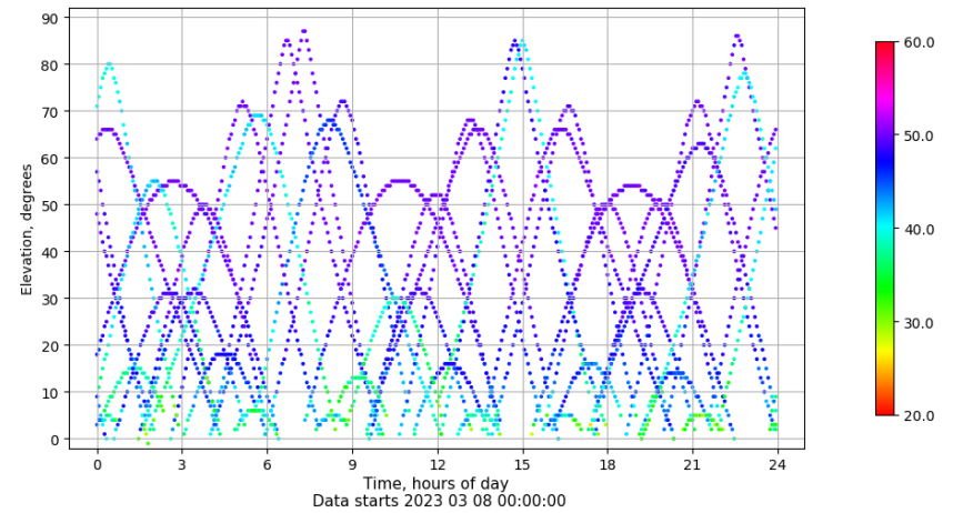
Time-elevation plot for station ZFRA. Signal to Noise S1C Data file ZFRA00ESP_R_2023067.xtr
