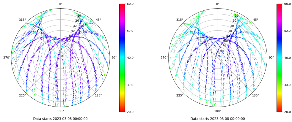
Skyplot for station ZFRA. Signal to Noise S1C Data file ZFRA00ESP_R_2023067.xtr Skyplot for station ZFRA. Signal to Noise S2P Data file ZFRA00ESP_R_2023067.xtr
