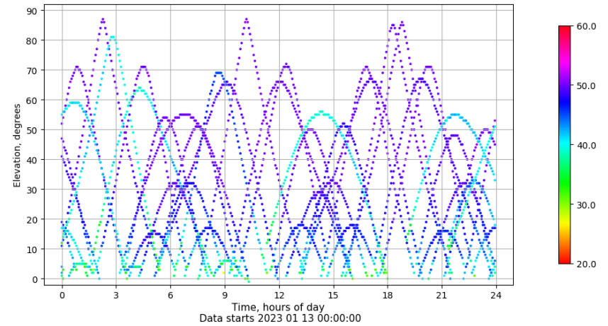
Time-elevation plot for station ZFRA. Signal to Noise S1C Data file ZFRA00ESP_R_2023013.xtr
