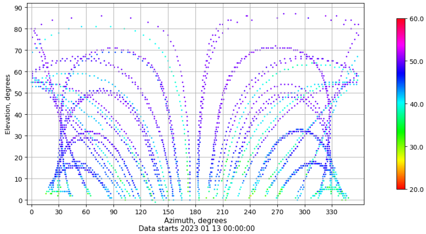
Azimuth-elevation plot for station ZFRA. Signal to Noise S1C Data file ZFRA00ESP_R_2023013.xtr
