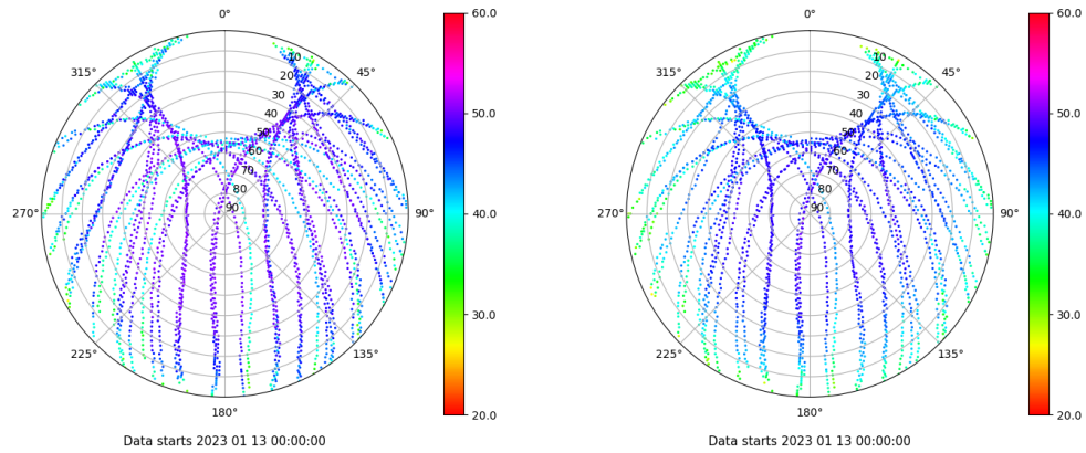
Skyplot for station ZFRA. Signal to Noise S1C Data file ZFRA00ESP_R_2023013.xtr Skyplot for station ZFRA. Signal to Noise S2P Data file ZFRA00ESP_R_2023013.xtr
