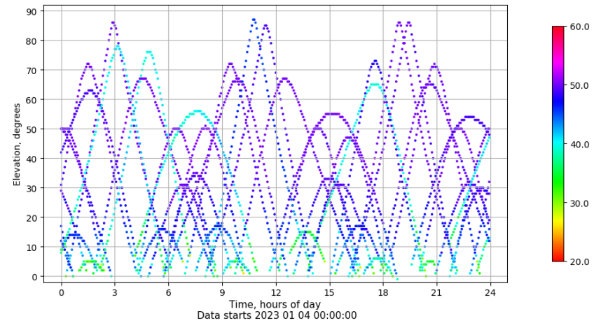
Time-elevation plot for station ZFRA. Signal to Noise S1C Data file ZFRA00ESP_R_2023004.xtr
