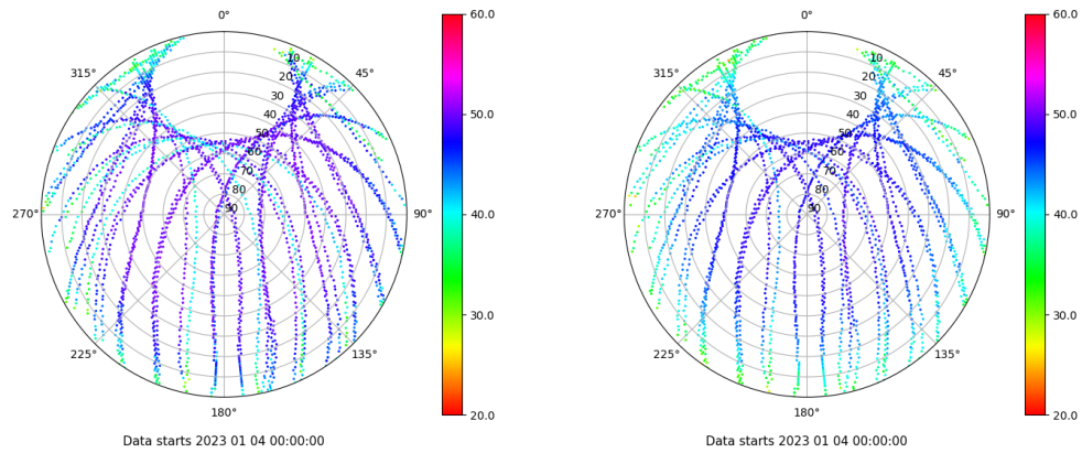
Skyplot for station ZFRA. Signal to Noise S1C Data file ZFRA00ESP_R_2023004.xtr Skyplot for station ZFRA. Signal to Noise S2P Data file ZFRA00ESP_R_2023004.xtr
