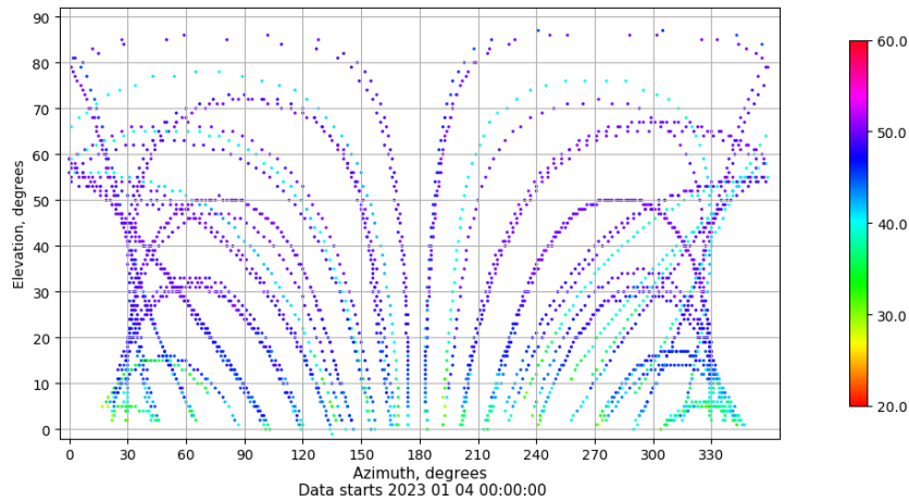
Azimuth-elevation plot for station ZFRA. Signal to Noise S1C Data file ZFRA00ESP_R_2023004.xtr
