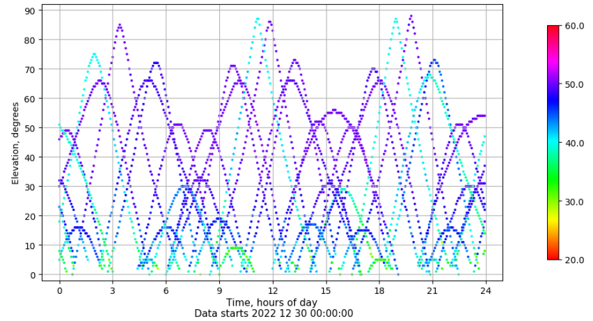
Time-elevation plot for station ZFRA. Signal to Noise S1C Data file ZFRA00ESP_R_2022364.xtr
