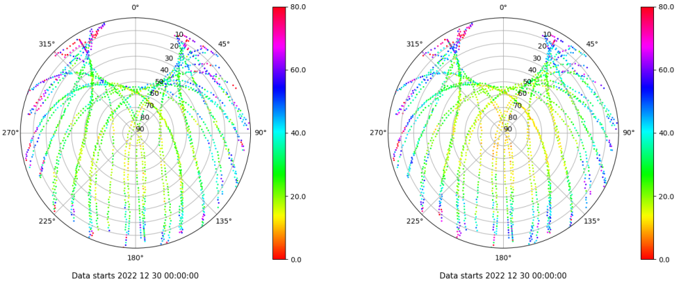
Skyplot for station ZFRA. Parameter M1C Data file ZFRA00ESP_R_2022364.xtr Skyplot for station ZFRA. Parameter M2P Data file ZFRA00ESP_R_2022364.xtr
