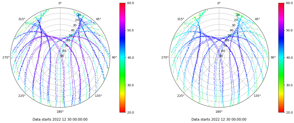
Skyplot for station ZFRA. Signal to Noise S1C Data file ZFRA00ESP_R_2022364.xtr Skyplot for station ZFRA. Signal to Noise S2P Data file ZFRA00ESP_R_2022364.xtr
