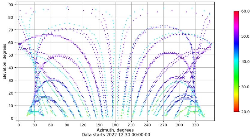
Azimuth-elevation plot for station ZFRA. Signal to Noise S1C Data file ZFRA00ESP_R_2022364.xtr
