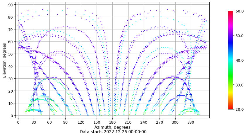
Azimuth-elevation plot for station ZFRA. Signal to Noise S1C Data file ZFRA00ESP_R_2022360.xtr
