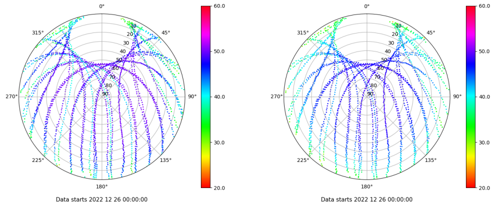
Skyplot for station ZFRA. Signal to Noise S1C Data file ZFRA00ESP_R_2022360.xtr Skyplot for station ZFRA. Signal to Noise S2P Data file ZFRA00ESP_R_2022360.xtr
