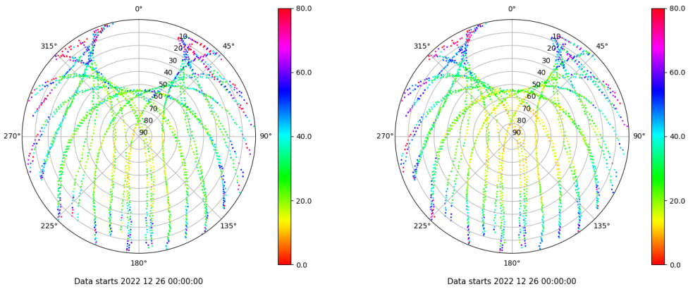
Skyplot for station ZFRA. Parameter M1C Data file ZFRA00ESP_R_2022360.xtr Skyplot for station ZFRA. Parameter M2P Data file ZFRA00ESP_R_2022360.xtr
