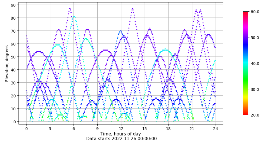
Time-elevation plot for station ZFRA. Signal to Noise S1C Data file ZFRA00ESP_R_2022330.xtr
