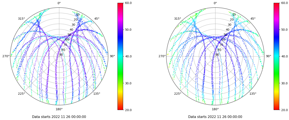
Skyplot for station ZFRA. Signal to Noise S1C Data file ZFRA00ESP_R_2022330.xtr Skyplot for station ZFRA. Signal to Noise S2P Data file ZFRA00ESP_R_2022330.xtr
