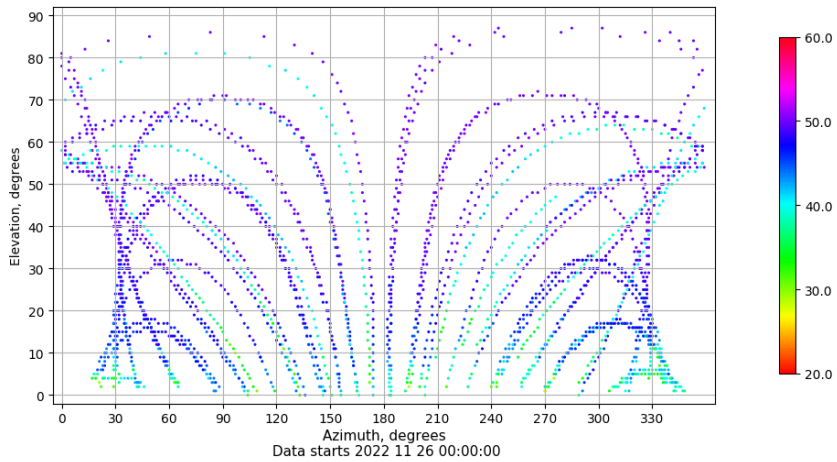
Azimuth-elevation plot for station ZFRA. Signal to Noise S1C Data file ZFRA00ESP_R_2022330.xtr
