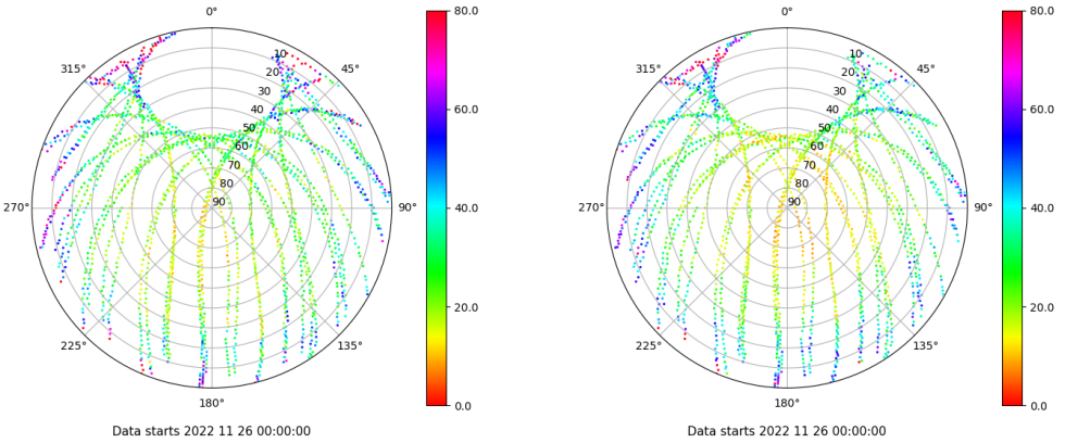
Skyplot for station ZFRA. Parameter M1C Data file ZFRA00ESP_R_2022330.xtr Skyplot for station ZFRA. Parameter M2P Data file ZFRA00ESP_R_2022330.xtr
