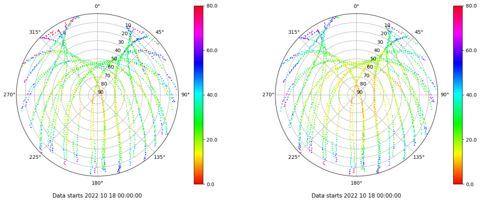
Skyplot for station ZFRA. Parameter M1C Data file ZFRA00ESP_R_2022291.xtr Skyplot for station ZFRA. Parameter M2P Data file ZFRA00ESP_R_2022291.xtr
