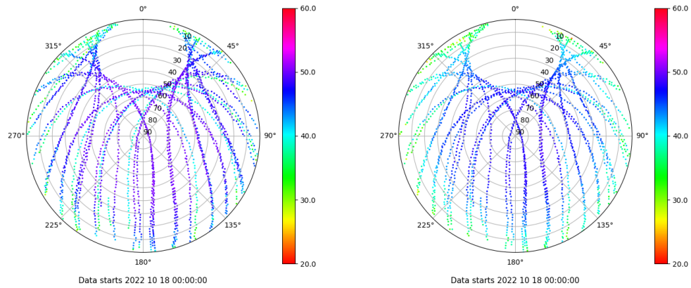
Skyplot for station ZFRA. Signal to Noise S1C Data file ZFRA00ESP_R_2022291.xtr Skyplot for station ZFRA. Signal to Noise S2P Data file ZFRA00ESP_R_2022291.xtr
