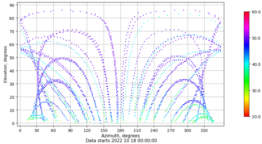
Azimuth-elevation plot for station ZFRA. Signal to Noise S1C Data file ZFRA00ESP_R_2022291.xtr
