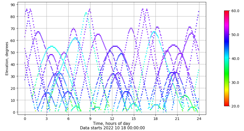
Time-elevation plot for station ZFRA. Signal to Noise S1C Data file ZFRA00ESP_R_2022291.xtr
