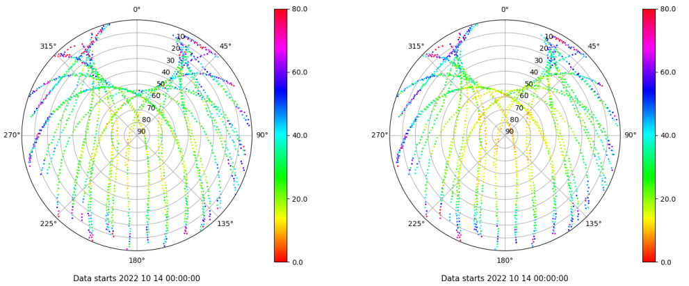
Skyplot for station ZFRA. Parameter M1C Data file ZFRA00ESP_R_2022287.xtr Skyplot for station ZFRA. Parameter M2P Data file ZFRA00ESP_R_2022287.xtr
