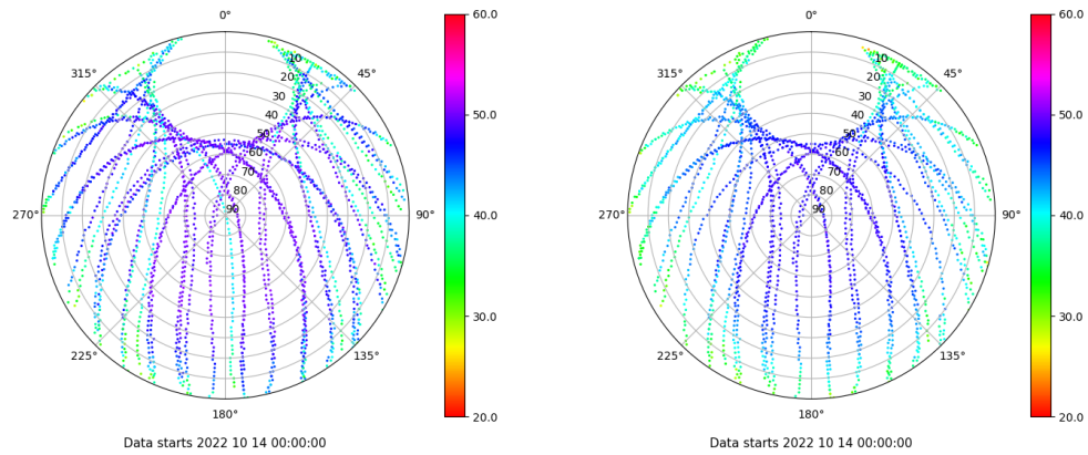
Skyplot for station ZFRA. Signal to Noise S1C Data file ZFRA00ESP_R_2022287.xtr Skyplot for station ZFRA. Signal to Noise S2P Data file ZFRA00ESP_R_2022287.xtr
