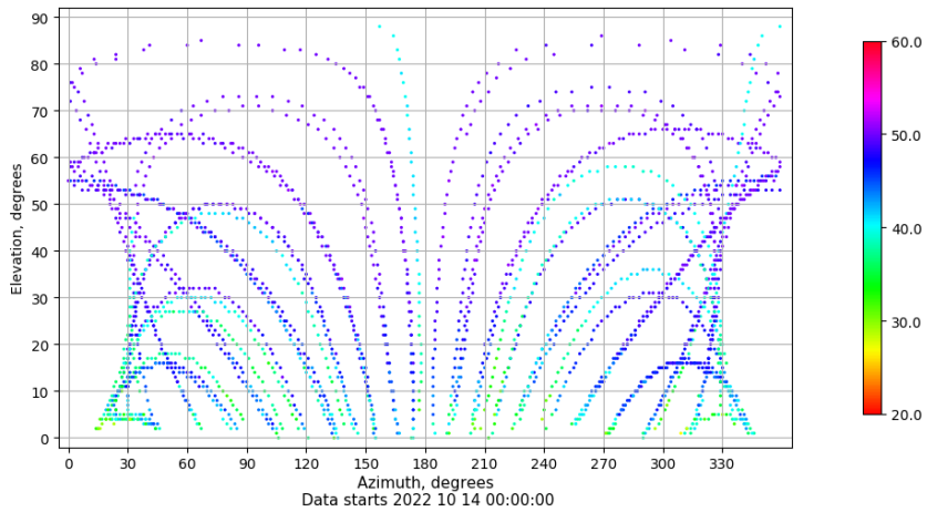
Azimuth-elevation plot for station ZFRA. Signal to Noise S1C Data file ZFRA00ESP_R_2022287.xtr
