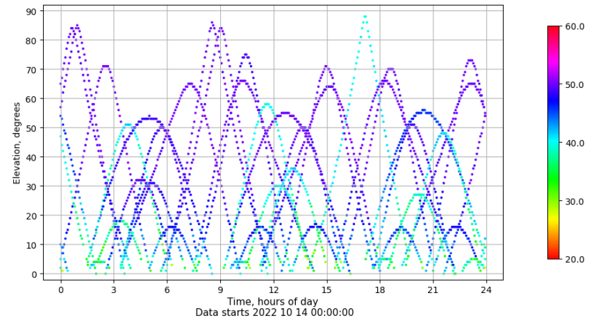
Time-elevation plot for station ZFRA. Signal to Noise S1C Data file ZFRA00ESP_R_2022287.xtr
