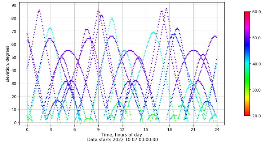
Time-elevation plot for station ZFRA. Signal to Noise S1C Data file ZFRA00ESP_R_2022280.xtr
