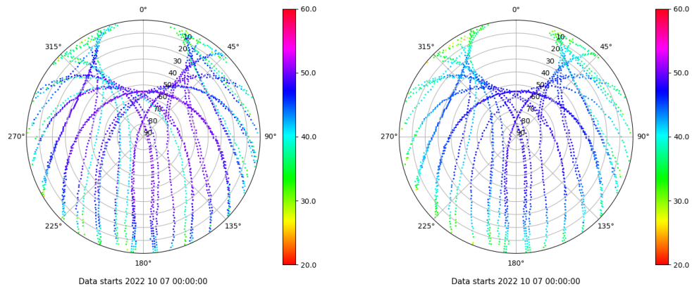
Skyplot for station ZFRA. Signal to Noise S1C Data file ZFRA00ESP_R_2022280.xtr Skyplot for station ZFRA. Signal to Noise S2P Data file ZFRA00ESP_R_2022280.xtr
