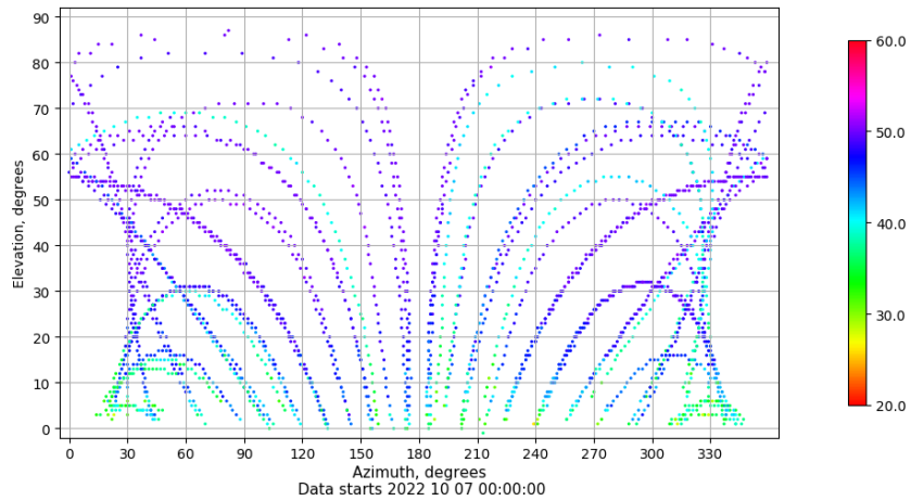
Azimuth-elevation plot for station ZFRA. Signal to Noise S1C Data file ZFRA00ESP_R_2022280.xtr
