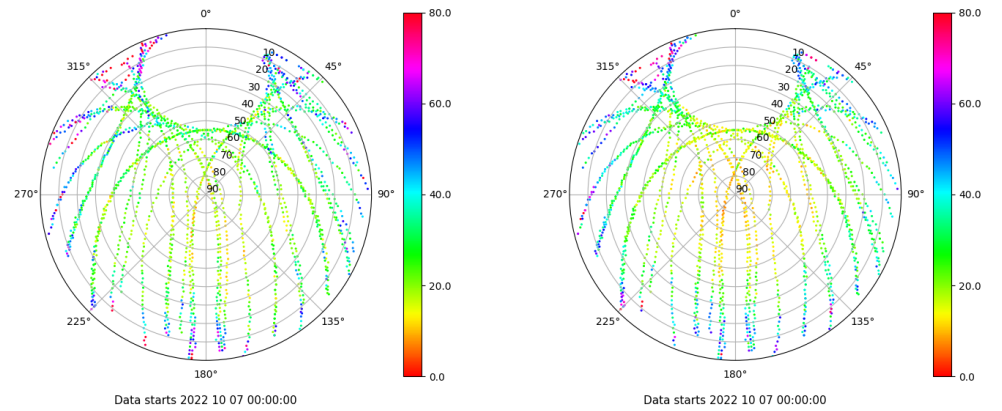
Skyplot for station ZFRA. Parameter M1C Data file ZFRA00ESP_R_2022280.xtr Skyplot for station ZFRA. Parameter M2P Data file ZFRA00ESP_R_2022280.xtr
